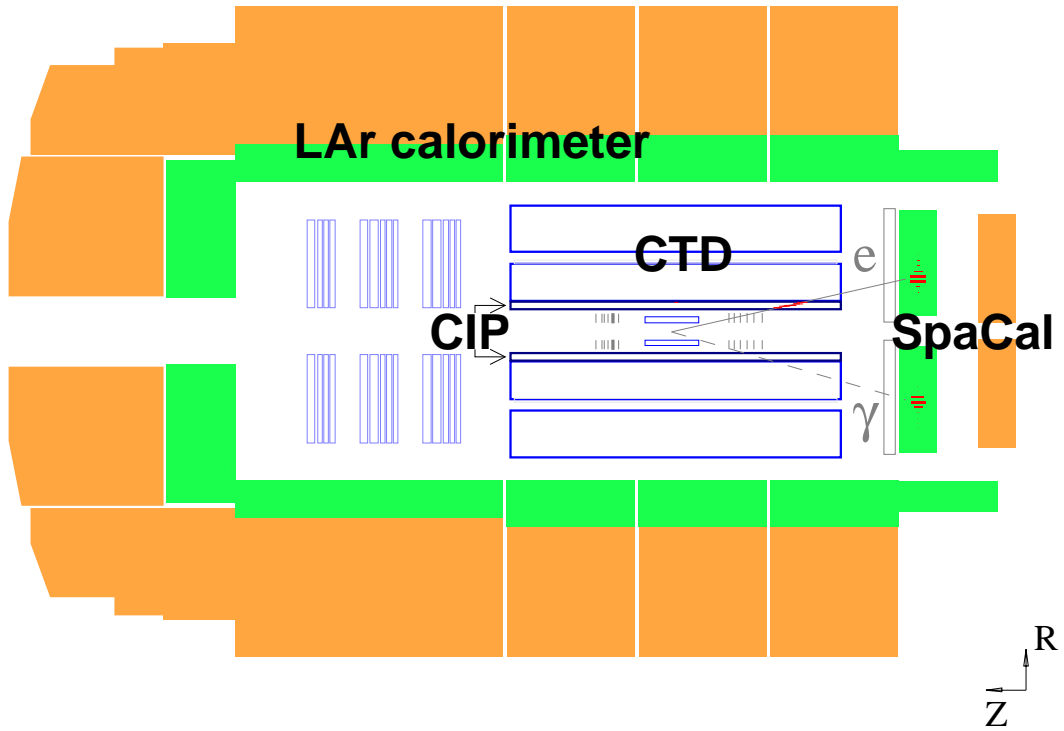
Figure 1: Elastic QEDC candidate event observed in the H1 detector. The H1 detector components most relevant to this analysis are indicated. The approximate electron and photon candidate trajectories are shown.
