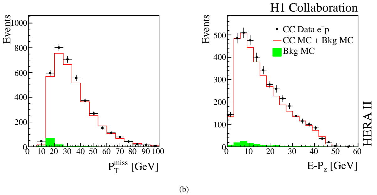
Figure 7: Distributions of P_T^{\text{miss}} and E - P_z for (a) e^-p and (b) e^+p CC data (solid points) and simulation (histograms). The estimated background contribution is shown as the shaded histograms.
