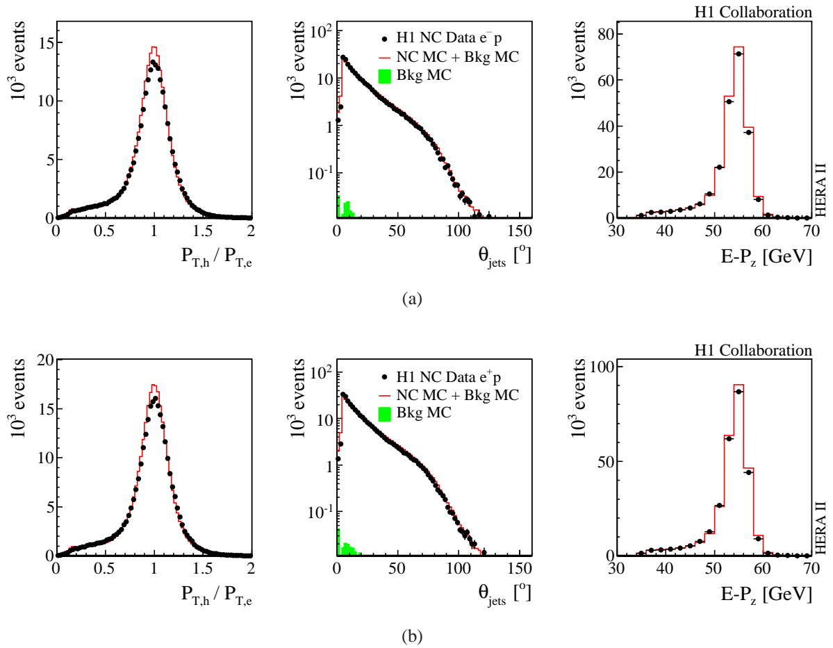
Figure 5: Distributions of P_{T,h}/P_{T,e} , \theta_{\text{jets}} and E - P_z in the region y < 0.19 for (a) e^-p and (b) e^+p data (solid points) and for simulation (histograms). The estimated background contribution is shown as the shaded histograms. The quantities P_{T,h} , \theta_{\text{jets}} and the hadronic contribution to E - P_z are calculated using energies associated within jets (see text).
