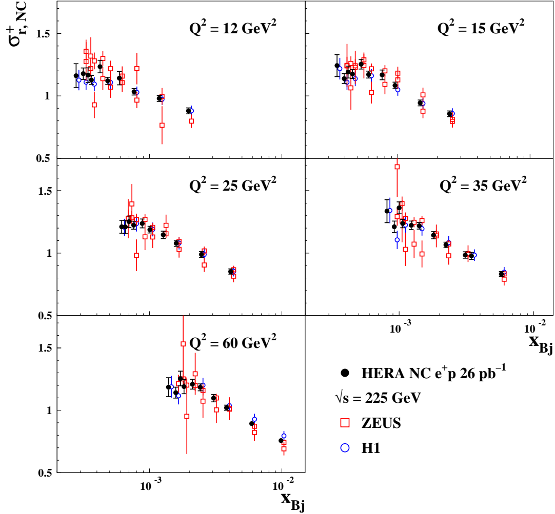
Figure 9: The combined HERA data for the inclusive NC e^+p reduced cross sections at \sqrt{s} = 225 \text{ GeV} as a function of x_{Bj} for five selected values of Q^2 compared to the individual H1 and ZEUS data. The individual measurements are displaced horizontally for better visibility. The ZEUS points at the same x_{Bj} and Q^2 values are from two different data sets. Error bars represent the total uncertainties.
