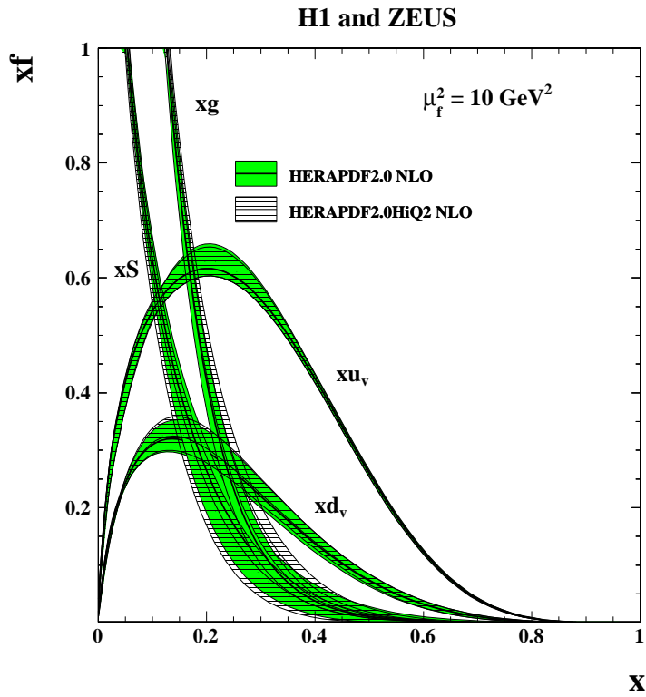
Figure 54: The parton distribution functions xu_v , xd_v , xS = 2x(\bar{U} + \bar{D}) and xg of HERAPDF2.0 NLO at \mu_f^2 = 10 \text{ GeV}^2 compared to those of HERAPDF2.0HiQ2 NLO on logarithmic (top) and linear (bottom) scales. The bands represent the total uncertainties.
