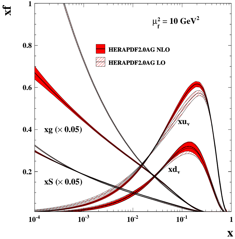
Figure 26: The parton distribution functions xu_v , xd_v , xS = 2x(\bar{U} + \bar{D}) and xg of HERAPDF2.0AG LO at \mu_f^2 = 10 \text{ GeV}^2 compared to those of HERAPDF2.0AG NLO. The bands represent the experimental uncertainties only.
