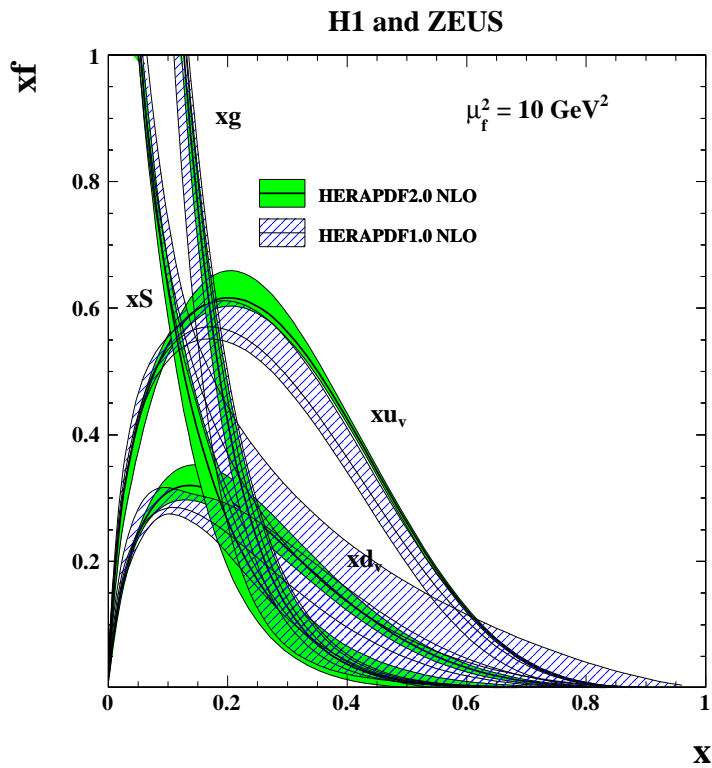
Figure 47: The parton distribution functions xu_v , xd_v , xS = 2x(\bar{U} + \bar{D}) and xg of HERAPDF2.0 NLO at \mu_f^2 = 10 \text{ GeV}^2 compared to those of HERAPDF1.0 on logarithmic (top) and linear (bottom) scales. The bands represent the total uncertainties.
