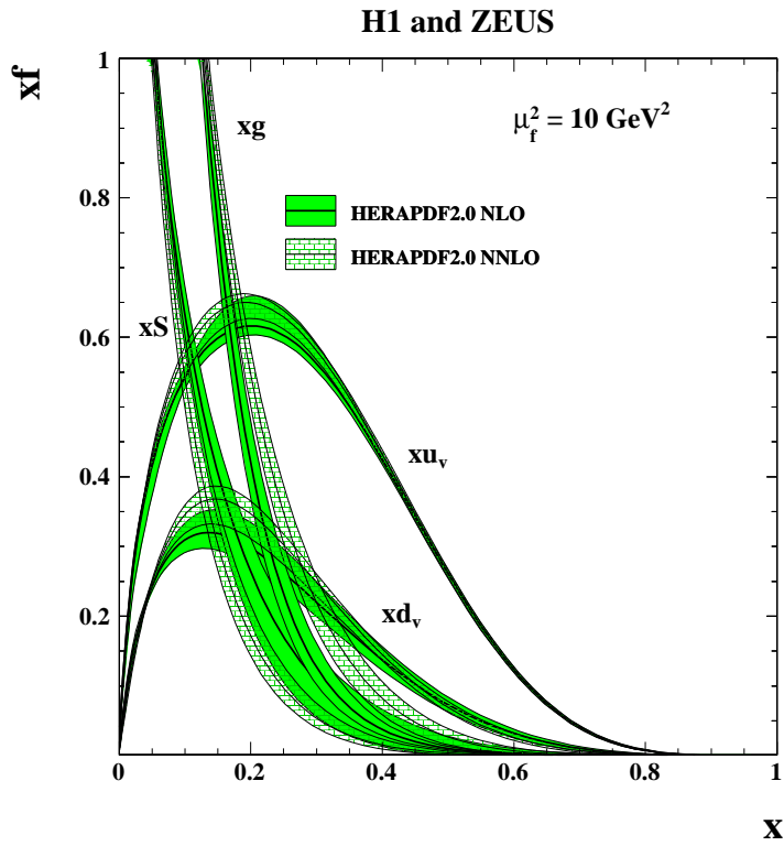
Figure 25: The parton distribution functions xu_v , xd_v , xS = 2x(\bar{U} + \bar{D}) and xg of HERAPDF2.0 NLO at \mu_f^2 = 10 \text{ GeV}^2 compared to those of HERAPDF2.0 NNLO on logarithmic (top) and linear (bottom) scales. The bands represent the total uncertainties.
