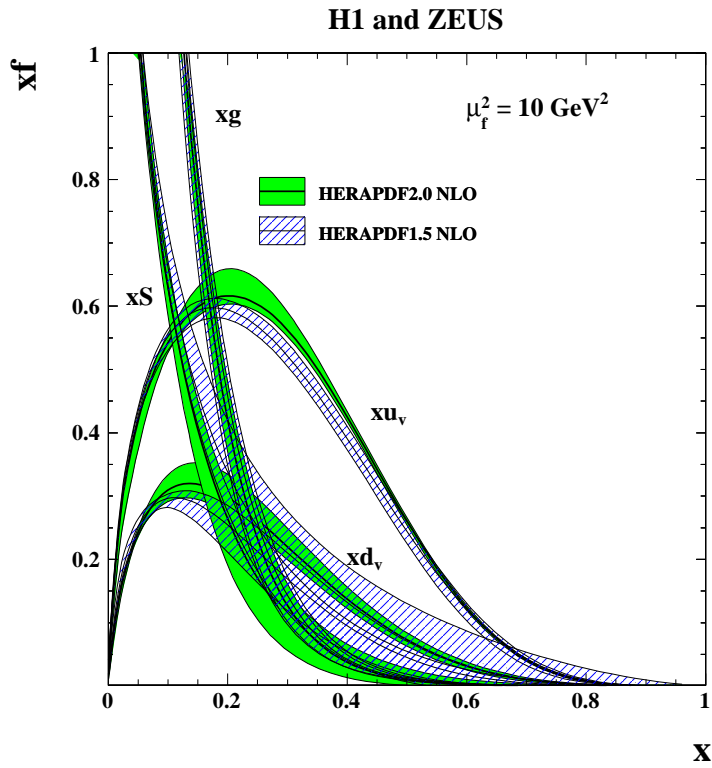
Figure 48: The parton distribution functions xu_v , xd_v , xS = 2x(\bar{U} + \bar{D}) and xg of HERAPDF2.0 NLO at \mu_f^2 = 10 \text{ GeV}^2 compared to those of HERAPDF1.5 on logarithmic (top) and linear (bottom) scales. The bands represent the total uncertainties.
