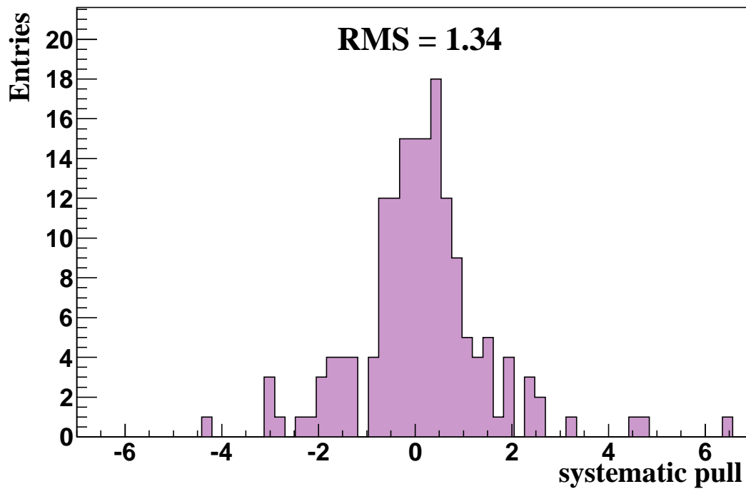
Figure 3: Distribution of pulls p_j for the correlated systematic uncertainties including global normalisations. There are no entries outside the histogram range. The root mean square, RMS, of the distribution is given.
