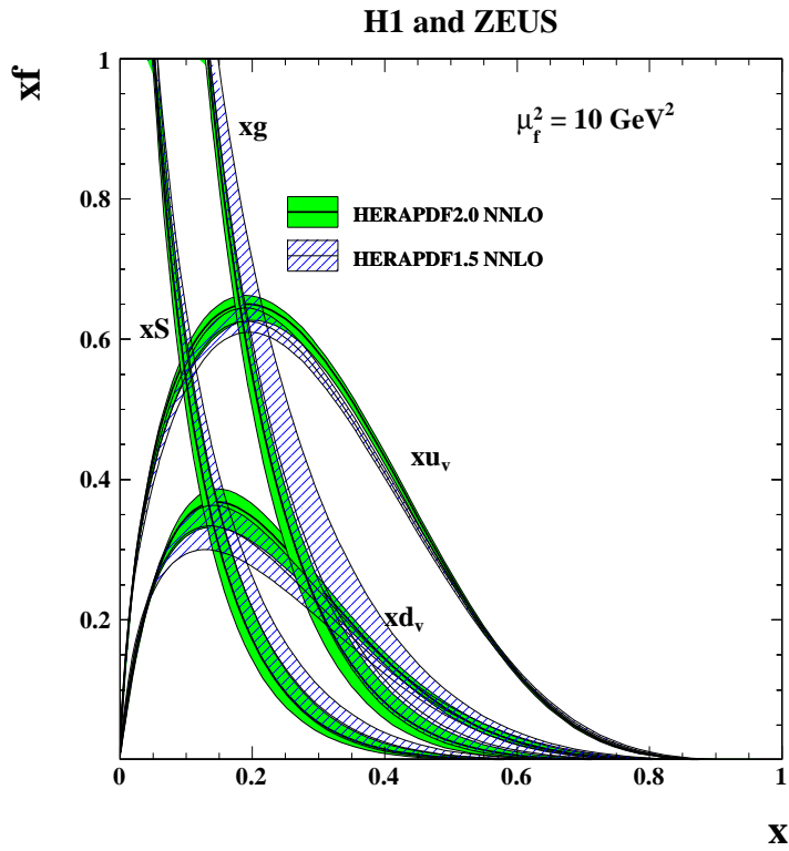
Figure 49: The parton distribution functions xu_v , xd_v , xS = 2x(\bar{U} + \bar{D}) and xg of HERAPDF2.0 NNLO at \mu_f^2 = 10 \text{ GeV}^2 compared to the ones of HERAPDF1.5 on logarithmic (top) and linear (bottom) scales. The bands represent the total uncertainties.
