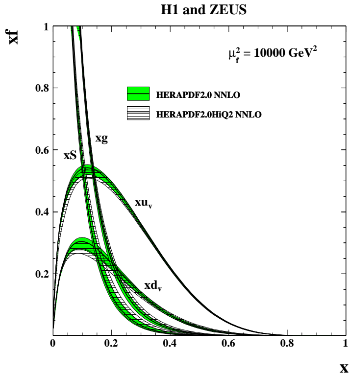
Figure 57: The parton distribution functions xu_v , xd_v , xS = 2x(\bar{U} + \bar{D}) and xg of HERAPDF2.0 NNLO at \mu_f^2 = 10000 \text{ GeV}^2 compared to those of HERAPDF2.0HiQ2 NNLO on logarithmic (top) and linear (bottom) scales. The bands represent the total uncertainties.
