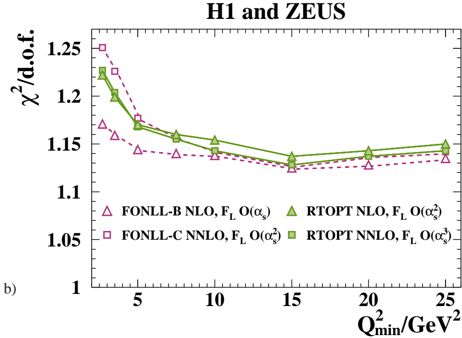
Figure 20: The dependence of \chi^2/\text{d.o.f.} on Q_{\min}^2 for HERAPDF2.0 fits using a) the RTOPT [84], FONLL-B [91], ACOT [110] and fixed-flavour (FF) schemes at NLO and b) the RTOPT and FONLL-B/C [92] schemes at NLO and NNLO. The F_L contributions are calculated using matrix elements of the order of \alpha_s indicated in the legend. The number of degrees of freedom drops from 1148 for Q_{\min}^2 = 2.7 \text{ GeV}^2 to 1131 for the nominal Q_{\min}^2 = 3.5 \text{ GeV}^2 and to 868 for Q_{\min}^2 = 25 \text{ GeV}^2 .
