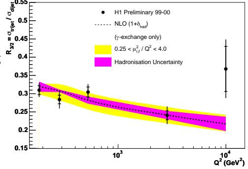
Figure 2: Trijet/dijet production ratio R_{3/2} (H1)
