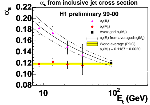
Figure 3: Running \alpha_S(E_{T,B}) from inclusive jet \sigma
