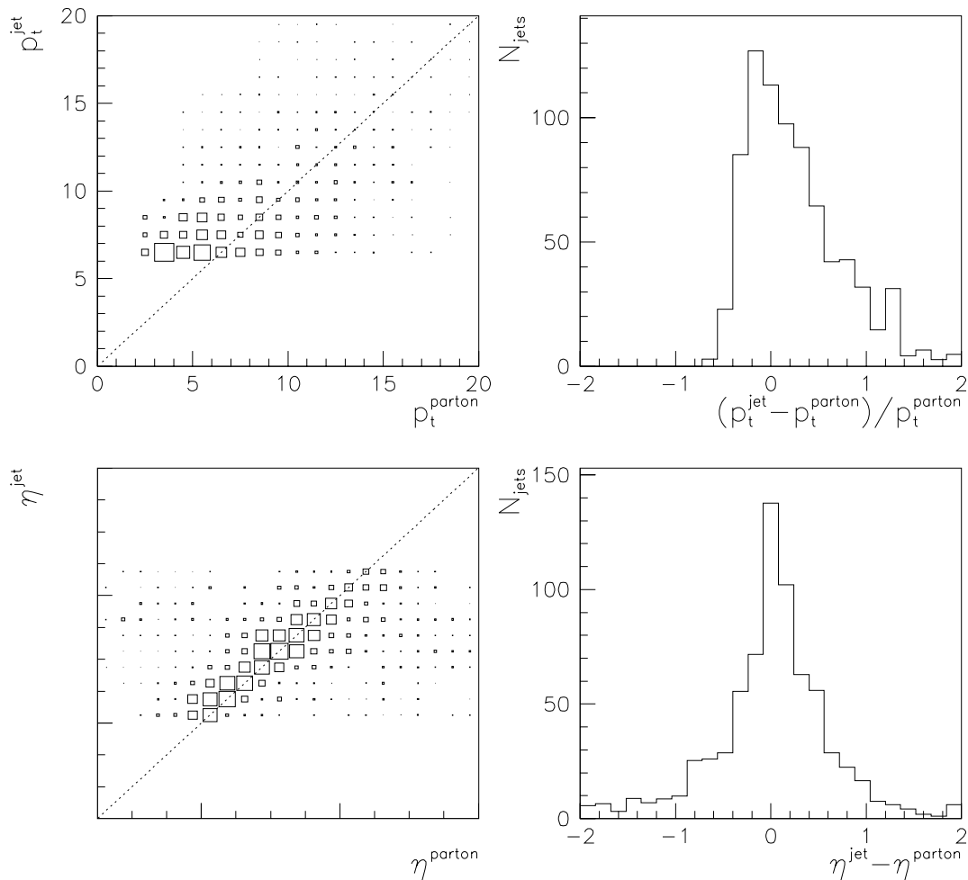
Figure 7.1: Jet parton correlation (LO) for p_t and \eta .
