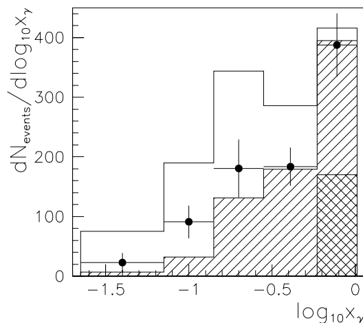
Figure 7.15: Unfolded \log_{10}x_\gamma -distribution. Comparison of data (points) and MC (histogram; the MC is normalized to the integrated luminosity of the data sample). The contributions to the x_\gamma -distribution due to direct (double hatched) and resolved processes are given separately (MC only). The latter are further subdivided into processes initiated by a quark (single hatched) or a gluon (open histogram) from the photon. The final, pedestal subtracted samples are used.
