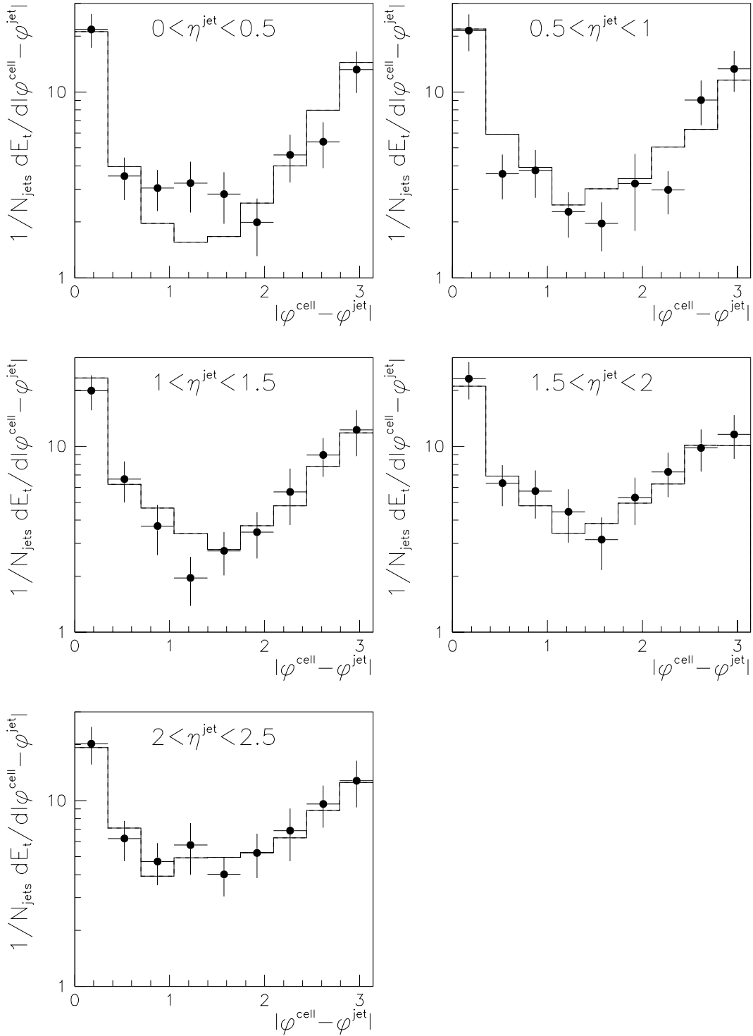
Figure 6.21: Jet-profiles in \varphi as a function of \eta^{\text{jet}} for \delta_{\text{cut}} = 0.05 . Jets are selected with 6 \text{ GeV}/c < p_t^{\text{jet}} < 8 \text{ GeV}/c . Data (points) is compared with a Monte Carlo simulation that includes multiple interactions (full histogram).
