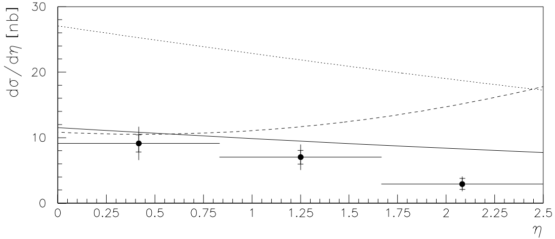
Figure 7.11: Inclusive parton cross-section d\sigma/d\eta in ep scattering versus the pseudorapidity \eta for \sqrt{s_{ep}} = 296 \text{ GeV} , Q^2 < 0.01 \text{ GeV}^2 , 0.25 < y < 0.7 and p_t > 6 \text{ GeV}/c determined for the pedestal subtracted sample. Inner error-bars show statistical errors, whereas outer error-bars are the (square root of the) quadratic sum of statistical and systematic errors, thereby neglecting the systematic error \sigma_{\text{others}} of 29.5%. The unfolding is performed by means of a Monte Carlo simulation which is based on leading order (partonic) matrix elements (see text). Comparison with theoretical predictions using the parton density function parametrizations of the photon by Glück, Reya and Vogt (GRV-LO, full line) and Abramowicz, Charchuła and Levy (LAC I, dashed line; LAC III, dotted line).
