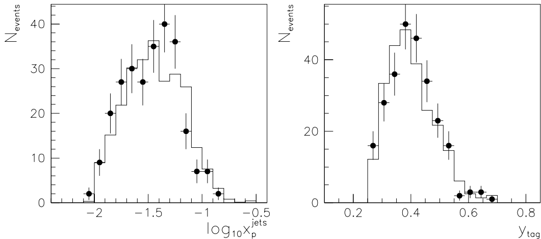
Figure 7.18: \log_{10}x_p^{\text{jets}} - and y_{\text{tag}} -distribution. Comparison of data (points) and reweighted Monte Carlo distribution (histogram). The MC is normalized to the integrated luminosity of the data sample. The final, pedestal subtracted samples are used.
