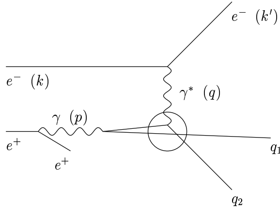
Figure 1.3: \gamma^* \gamma \rightarrow q_1 q_2 .
