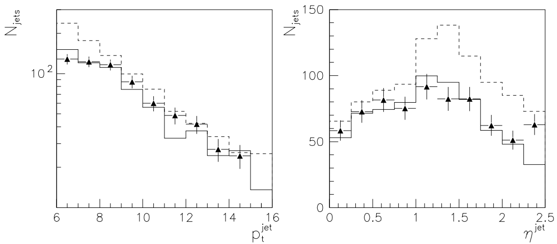
Figure 6.12: p_t^{\text{jet}} - and \eta^{\text{jet}} -distribution for different MC samples. Shown are the distributions for the MC without additional interactions (triangles) together with the distributions for the MC that includes multiple interactions before (dashed histogram) and after (full histogram) the pedestal subtraction. All distributions are normalized to the same integrated luminosity and have a cut applied at \hat{p}_t = 4 \text{ GeV}/c .
