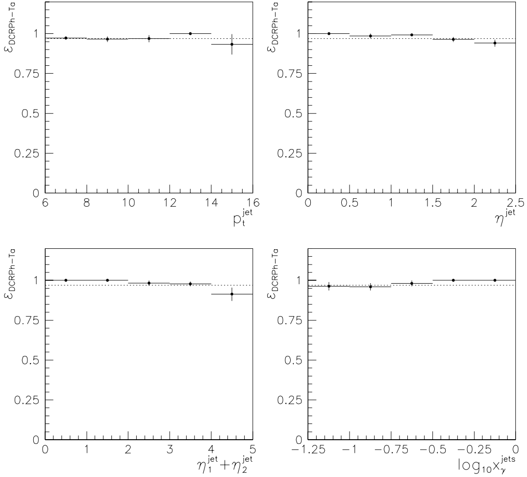
Figure 5.1: Efficiency of the DCRPh-Ta trigger-element as a function of p_t^{\text{jet}} , \eta^{\text{jet}} , \eta_1^{\text{jet}} + \eta_2^{\text{jet}} and \log_{10} x_\gamma^{\text{jets}} . The dotted line indicates the average efficiency of 97%.
