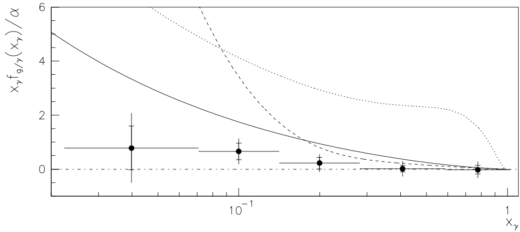
Figure 7.20: Momentum weighted gluon density function x_\gamma f_{g/\gamma}(x_\gamma, \mu^2)/\alpha of the photon at \mu^2 = \langle \hat{p}_t \rangle^2 = 75 \text{ GeV}^2 determined with the pedestal subtracted sample. Inner error-bars show statistical errors, whereas outer error-bars are the (square root of the) quadratic sum of statistical and systematic errors. Comparison with the parametrizations of Glück, Reya and Vogt (GRV-LO, full line) and Abramowicz, Charchuła and Levy (LAC I, dashed line; LAC III, dotted line).
