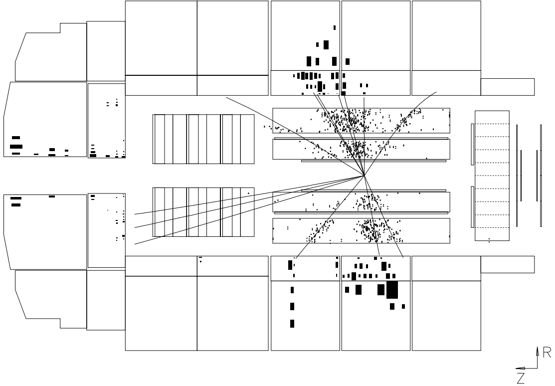
Figure 5.5: 2-jet event. Candidate for a direct photoproduction event. Depicted is a cross-section of the H1 detector along the z -axis, showing the liquid argon calorimeter, the BEMC and the tracking chambers. The measured energy in the LAr calorimeter and the BEMC is represented by black squares. The size of the squares is thereby proportional to the deposited energy. Additionally shown are the hits in the central tracking chambers together with the reconstructed particle tracks.
