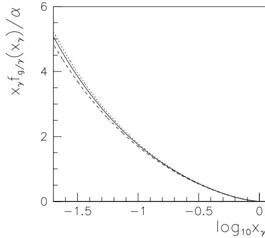
Figure 7.19: Momentum weighted gluon density function x_\gamma f_{g/\gamma}(x_\gamma, \mu^2)/\alpha of the photon for different scales \mu^2 = \langle \hat{p}_t \rangle^2 . Comparison of the GRV-LO parametrization for \mu^2 = 75 \text{ GeV}^2 (full line), \mu^2 = 50 \text{ GeV}^2 (dashed line) and \mu^2 = 100 \text{ GeV}^2 (dotted line).
