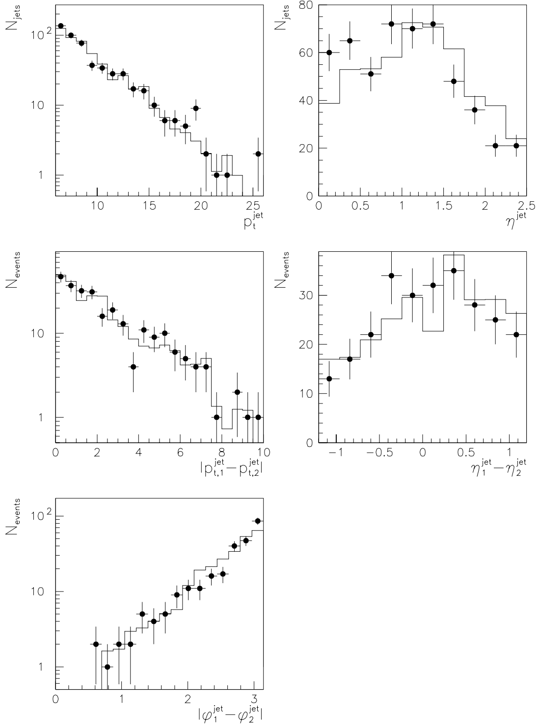
Figure 7.6: p_t^{\text{jet}} , \eta^{\text{jet}} , |p_{t,1}^{\text{jet}} - p_{t,2}^{\text{jet}}| , \eta_1^{\text{jet}} - \eta_2^{\text{jet}} and |\varphi_1^{\text{jet}} - \varphi_2^{\text{jet}}| distribution. Comparison of data (points) and reweighted Monte Carlo distribution (histogram). The MC is normalized to the integrated luminosity of the data sample. The final, pedestal subtracted samples are used.
