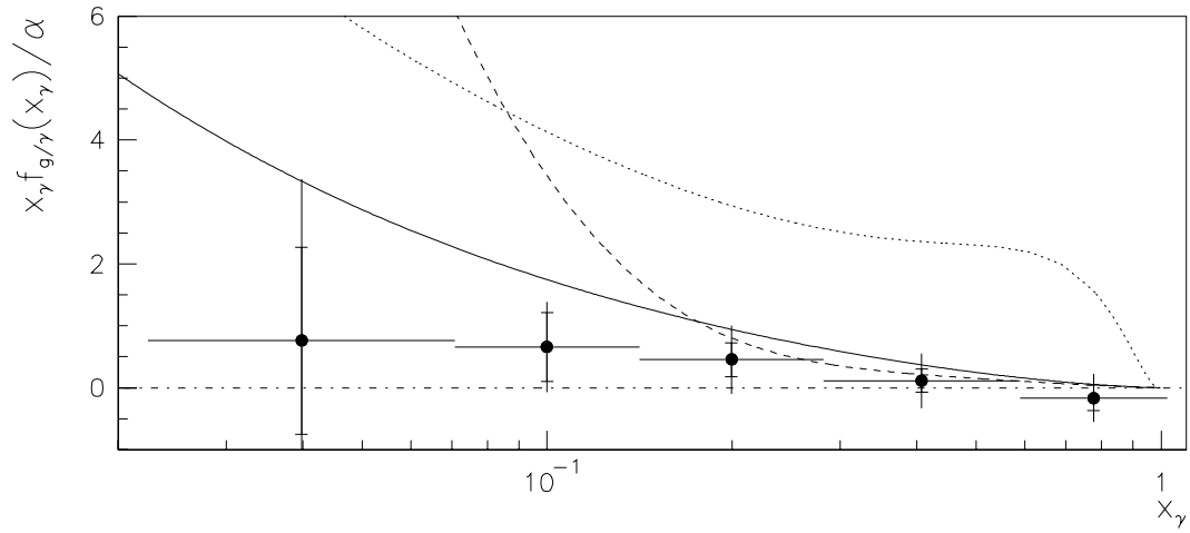
Figure 7.22: Momentum weighted gluon density function x_\gamma f_{g/\gamma}(x_\gamma, \mu^2)/\alpha of the photon at \mu^2 = \langle \hat{p}_t \rangle^2 = 75 \text{ GeV}^2 determined with the sub-jet sample. Inner error-bars show statistical errors, whereas outer error-bars are the (square root of the) quadratic sum of statistical and systematic errors. Comparison with the parametrizations of Glück, Reya and Vogt (GRV-LO, full line) and Abramowicz, Charchuła and Levy (LAC I, dashed line; LAC III, dotted line).
