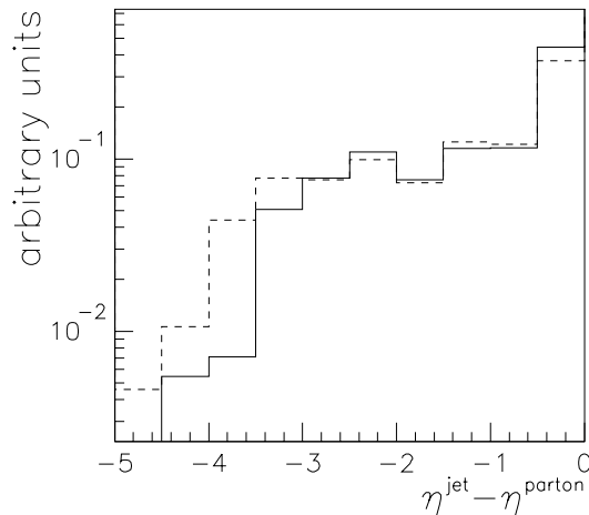
Figure 4.4: Jet parton correlation for \eta at low x_{\gamma} ( x_{\gamma} < 0.1 ) before (dashed line) and after (full line) applying the cut on |\Delta\eta^{\text{jets}}| . Both distributions are normalized to unit area.
