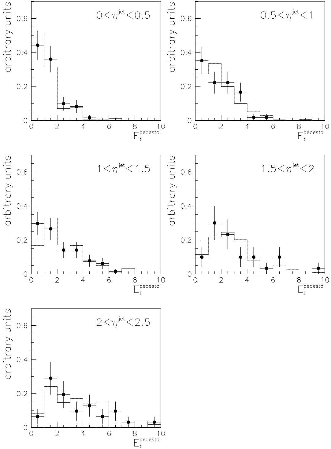
Figure 6.22: E_t^{\text{pedestal}} -distribution as a function of \eta^{\text{jet}} for \delta_{\text{cut}} = 0.05 . Comparison of data (points) and MC (histogram). The MC sample used includes multiple interactions. The distributions are normalized to unit area.
