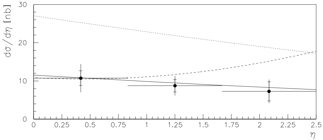
Figure 7.13: Inclusive parton cross-section d\sigma/d\eta in ep scattering versus the pseudo-rapidity \eta for \sqrt{s_{ep}} = 296 \text{ GeV} , Q^2 < 0.01 \text{ GeV}^2 , 0.25 < y < 0.7 and p_t > 6 \text{ GeV}/c determined for the sub-jet sample. Inner error-bars show statistical errors, whereas outer error-bars are the (square root of the) quadratic sum of statistical and systematic errors, thereby neglecting the systematic error \sigma_{\text{others}} of 29.5%. The unfolding is performed by means of a Monte Carlo simulation which is based on leading order (partonic) matrix elements (see text). Comparison with theoretical predictions using the parton density function parametrizations of the photon by Glück, Reya and Vogt (GRV-LO, full line) and Abramowicz, Charchuła and Levy (LAC I, dashed line; LAC III, dotted line).
