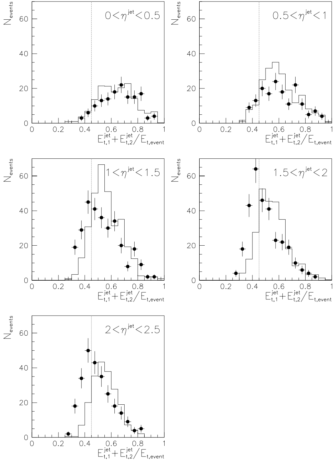
Figure 6.17: (E_{t,1}^{\text{jet}} + E_{t,2}^{\text{jet}})/E_{t,\text{event}} -distribution as a function of \eta^{\text{jet}} . Comparison of data (points) and MC (histogram; the MC is normalized to the integrated luminosity of the data sample). The MC sample used includes multiple interactions. The dotted line indicates the cut applied.
