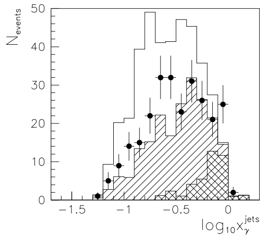
Figure 7.3: \log_{10}x_{\gamma}^{\text{jets}} -distribution. Comparison of data (points) and MC (histogram; the MC is normalized to the integrated luminosity of the data sample). The contributions to the x_{\gamma}^{\text{jets}} -distribution due to direct (double hatched) and resolved processes are given separately (MC only). The latter are further subdivided into processes initiated by a quark (single hatched) or a gluon (open histogram) from the photon. The final, pedestal subtracted samples are used.
