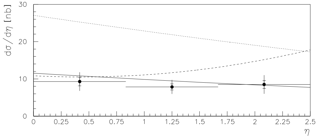
Figure 7.12: Inclusive parton cross-section d\sigma/d\eta in ep scattering versus the pseudorapidity \eta for \sqrt{s_{ep}} = 296 GeV, Q^2 < 0.01 GeV 2 , 0.25 < y < 0.7 and p_t > 6 GeV/c determined for the fluctuation reduced sample. Inner error-bars show statistical errors, whereas outer error-bars are the (square root of the) quadratic sum of statistical and systematic errors, thereby neglecting the systematic error \sigma_{\text{others}} of 29.5%. The unfolding is performed by means of a Monte Carlo simulation which is based on leading order (partonic) matrix elements (see text). Comparison with theoretical predictions using the parton density function parametrizations of the photon by Glück, Reya and Vogt (GRV-LO, full line) and Abramowicz, Charchuła and Levy (LAC I, dashed line; LAC III, dotted line).
