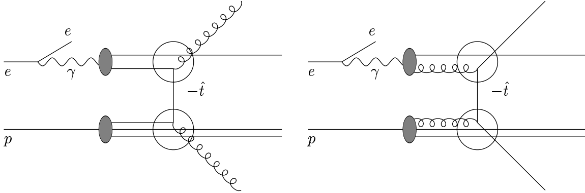
Figure 1.6: Two of the many possible resolved processes (LO QCD) in photon proton scattering.
