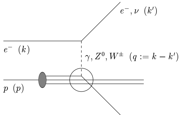
Figure 1.1: Kinematics of electron proton scattering. Henceforth, a shaded oval stands for a structured object and a transparent circle indicates an interaction with a parton from the extended object. Any lines emerging from either one are purely suggestive.
