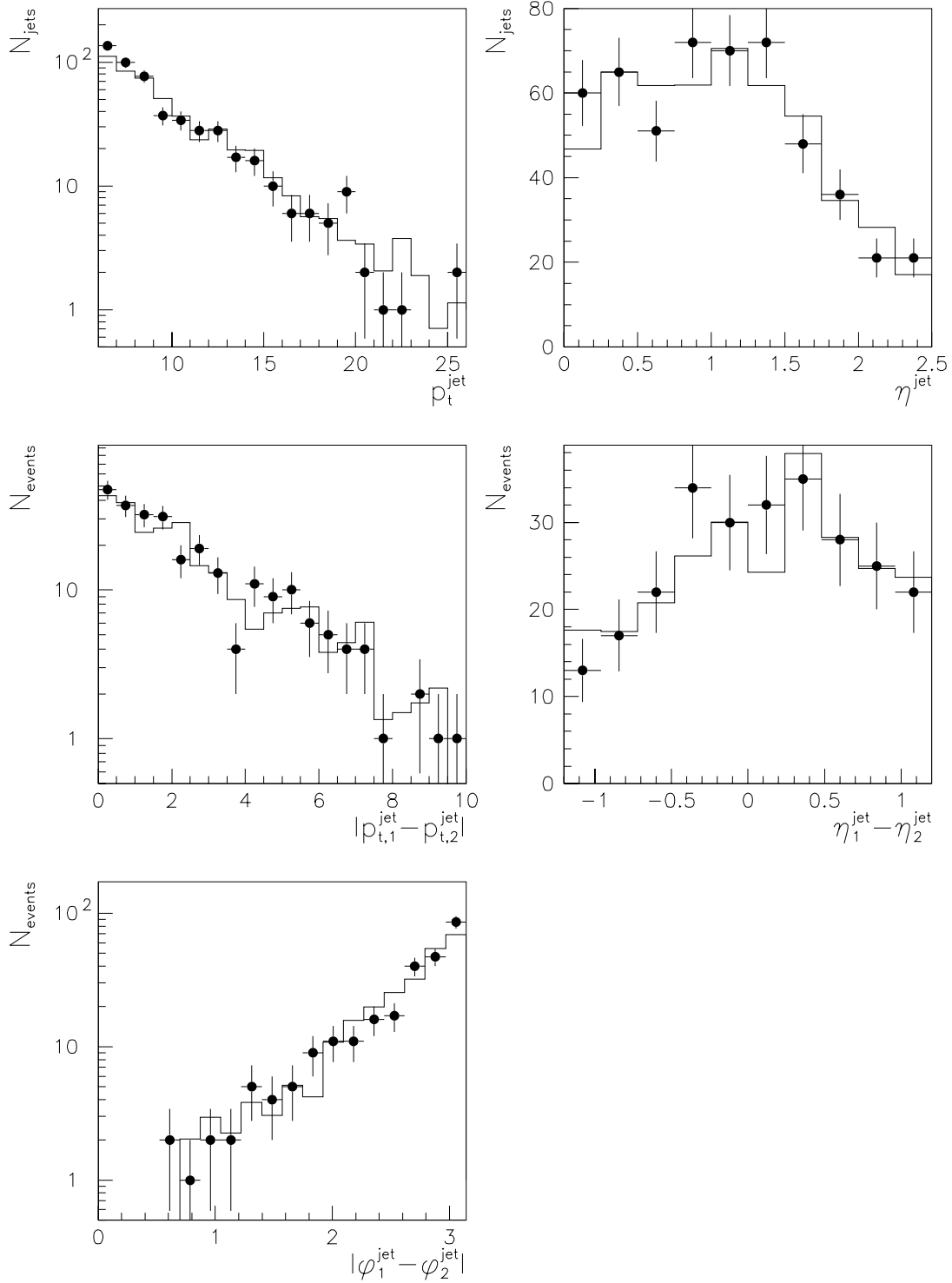
Figure 7.17: p_t^{\text{jet}} , \eta^{\text{jet}} , |p_{t,1}^{\text{jet}} - p_{t,2}^{\text{jet}}| , \eta_1^{\text{jet}} - \eta_2^{\text{jet}} and |\varphi_1^{\text{jet}} - \varphi_2^{\text{jet}}| distribution. Comparison of data (points) and reweighted Monte Carlo distribution (histogram). The MC is normalized to the integrated luminosity of the data sample. The final, pedestal subtracted samples are used.
