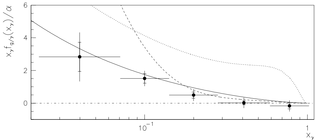
Figure 7.21: Momentum weighted gluon density function x_\gamma f_{g/\gamma}(x_\gamma, \mu^2)/\alpha of the photon at \mu^2 = \langle \hat{p}_t \rangle^2 = 75 \text{ GeV}^2 determined with the fluctuation reduced sample. Inner error-bars show statistical errors, whereas outer error-bars are the (square root of the) quadratic sum of statistical and systematic errors. Comparison with the parametrizations of Glück, Reya and Vogt (GRV-LO, full line) and Abramowicz, Charchuła and Levy (LAC I, dashed line; LAC III, dotted line).
