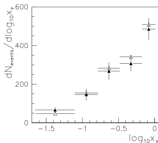
Figure 7.14: \log_{10}x_\gamma -distribution. Comparison of the unfolded d\tilde{N}_{\text{events}}(x_\gamma)/dx_\gamma -distribution ( \blacktriangle ) with the input distribution dN_{\text{events}}(x_\gamma)/dx_\gamma ( \Delta ).
