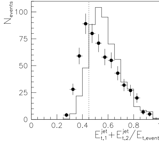
Figure 6.16: (E_{t,1}^{\text{jet}} + E_{t,2}^{\text{jet}})/E_{t,\text{event}} -distribution. Comparison of data (points) and MC (histogram; the MC is normalized to the integrated luminosity of the data sample). The MC sample used includes multiple interactions. The dotted line indicates the cut applied.
