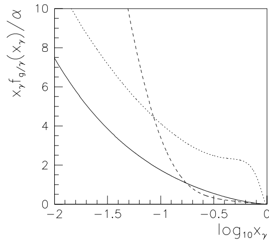
Figure 1.8: Different parametrizations of the momentum weighted gluon density function x_\gamma f_{g/\gamma}(x_\gamma, \mu^2)/\alpha . Comparison of the GRV-LO (full line), LAC I (dashed line) and LAC III (dotted line) parametrizations at \mu^2 = 75 \text{ GeV}^2 .
