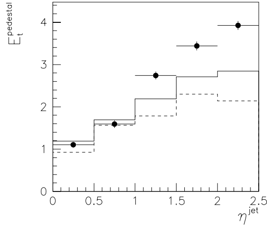
Figure 6.10: Average E_t^{\text{pedestal}} as a function of \eta^{\text{jet}} . Comparison of data (points) and Monte Carlo simulations (full histogram: including multiple interactions, dashed histogram: no additional interactions).
