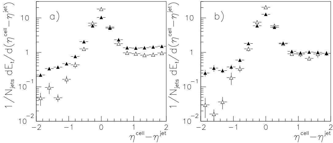
Figure 6.7: Jet-profile in \eta for the MC simulations. Transverse energy flow (per jet) around the jet direction in a slice of |\varphi^{\text{cell}} - \varphi^{\text{jet}}| < 1 versus the distance in \eta from the jet axis. Jets are selected with 0 < \eta^{\text{jet}} < 1 and the profiles are given for x_{\gamma}^{\text{jets}} < 0.5 ( \blacktriangle ) and x_{\gamma}^{\text{jets}} > 0.7 ( \triangle ). Figure a) shows the jet-profile for a MC simulation that includes multiple interactions whereas b) shows the profile for a MC simulation without additional soft interactions.
