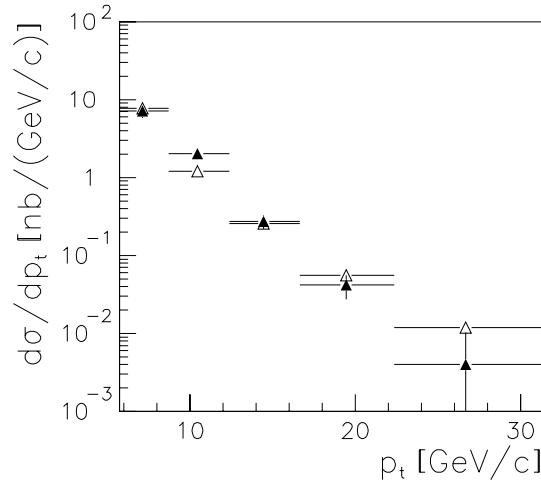
Figure 7.4: d\sigma(p_t)/dp_t -distribution. Comparison of the unfolded d\tilde{\sigma}(p_t)/dp_t -distribution ( \blacktriangle ) with the input distribution d\sigma(p_t)/dp_t ( \Delta ).
