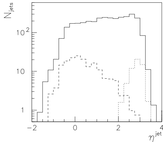
Figure 4.1: \eta^{\text{jet}} -distribution for jets ( E_t^{\text{jet}} > 6 GeV) which were successfully matched with a parton from the hard subprocess (full line) and for jets matched with the photon (dashed line) or proton (dotted line) remnant.
