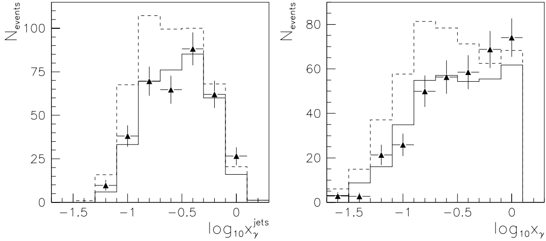
Figure 6.13: x_\gamma^{\text{jets}} - and x_\gamma -distribution for different MC samples. Shown are the distributions for the MC without additional interactions (triangles) together with the distributions for the MC that includes multiple interactions before (dashed histogram) and after (full histogram) the pedestal subtraction. All distributions are normalized to the same integrated luminosity and have a cut applied at \hat{p}_t = 4 \text{ GeV}/c .
