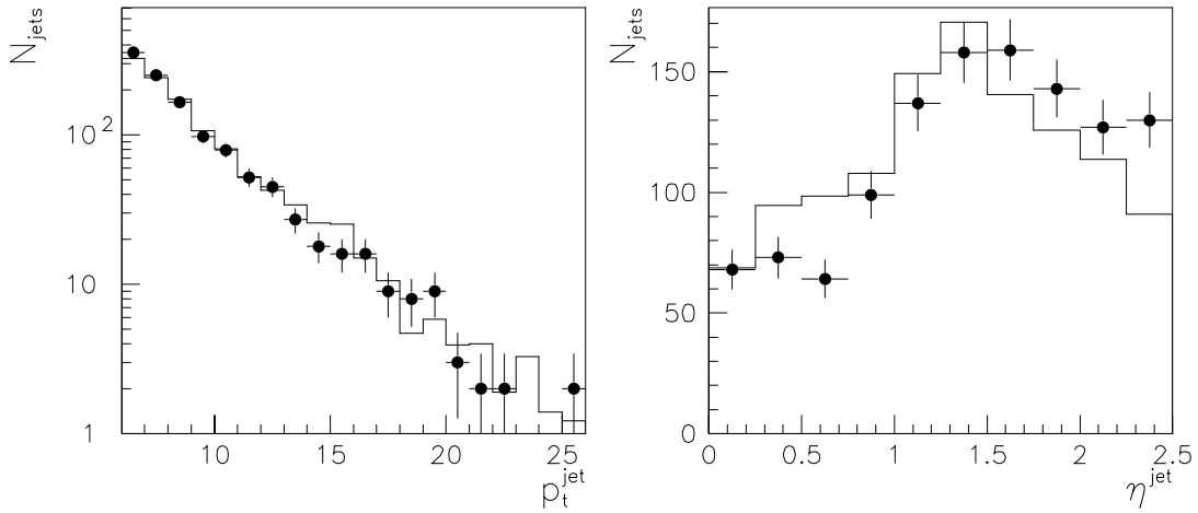
Figure 6.1: p_t^{\text{jet}} - and \eta^{\text{jet}} -distribution for 2-jet events. The number of jets found in the data sample (points) is compared with the absolute prediction of the Monte Carlo simulation (histogram; the MC is normalized to the integrated luminosity of the data sample). The MC sample used includes multiple interactions. We omit to plot the statistical errors for the MC simulations in this chapter in order not to overload the figures.
