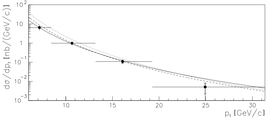
Figure 7.9: Inclusive parton cross-section d\sigma/dp_t in ep scattering versus the transverse momentum p_t for \sqrt{s_{ep}} = 296 GeV, Q^2 < 0.01 GeV 2 , 0.25 < y < 0.7 and 0 < \eta < 2.5 determined for the fluctuation reduced sample. Inner error-bars show statistical errors, whereas outer error-bars are the (square root of the) quadratic sum of statistical and systematic errors, thereby neglecting the systematic error \sigma_{\text{others}} of 29.5%. The unfolding is performed by means of a Monte Carlo simulation which is based on leading order (partonic) matrix elements (see text). Comparison with theoretical predictions using the parton density function parametrizations of the photon by Glück, Reya and Vogt (GRV-LO, full line) and Abramowicz, Charchuła and Levy (LAC I, dashed line; LAC III, dotted line).
