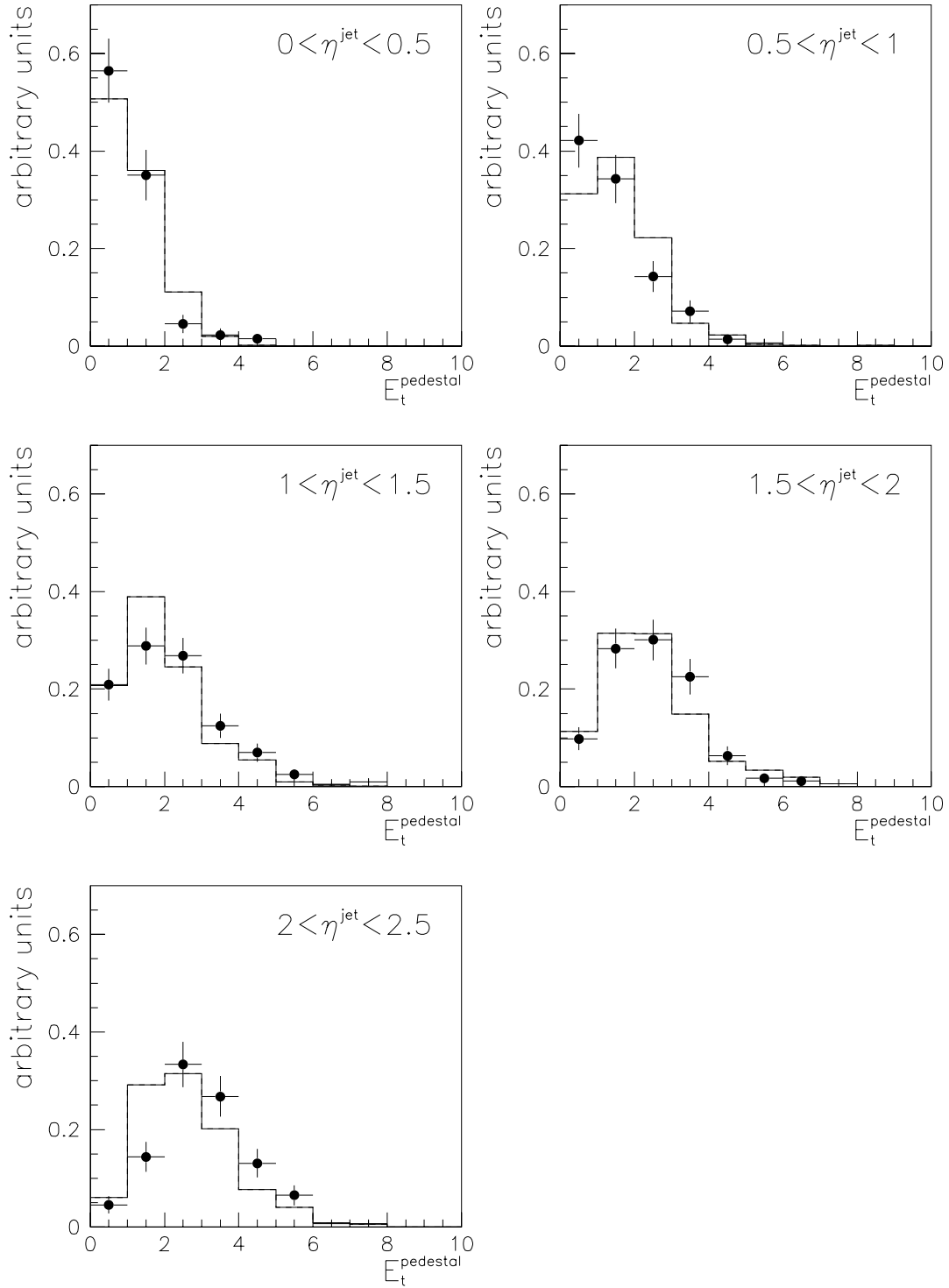
Figure 6.19: E_t^{\text{pedestal}} -distribution as a function of \eta^{\text{jet}} after the cut on (E_{t,1}^{\text{jet}} + E_{t,2}^{\text{jet}})/E_{t,\text{event}} . Comparison of data (points) and MC (histogram). The MC sample used includes multiple interactions. The distributions are normalized to unit area.
