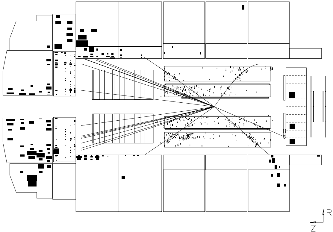
Figure 5.4: 2-jet event. Candidate for a resolved photoproduction event. Depicted is a cross-section of the H1 detector along the z -axis, showing the liquid argon calorimeter, the BEMC and the tracking chambers. The measured energy in the LAr calorimeter and the BEMC is represented by black squares. The size of the squares is thereby proportional to the deposited energy. Additionally shown are the hits in the central tracking chambers together with the reconstructed particle tracks.
