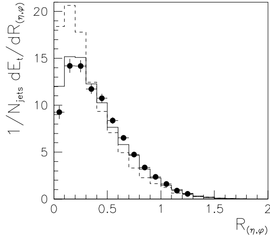
Figure 6.8: Transverse energy flow (per jet) as a function of R_{(\eta,\varphi)} ( R_{(\eta,\varphi)} := \sqrt{(\eta^{\text{cluster}} - \eta^{\text{jet}})^2 + (\varphi^{\text{cluster}} - \varphi^{\text{jet}})^2} ) for jets in the final data (points) and MC samples (full histogram: including multiple interactions, dashed histogram: no additional interactions). Only energy clusters which were assigned to the jet by the k_{\perp} -algorithm contribute to the plot.
