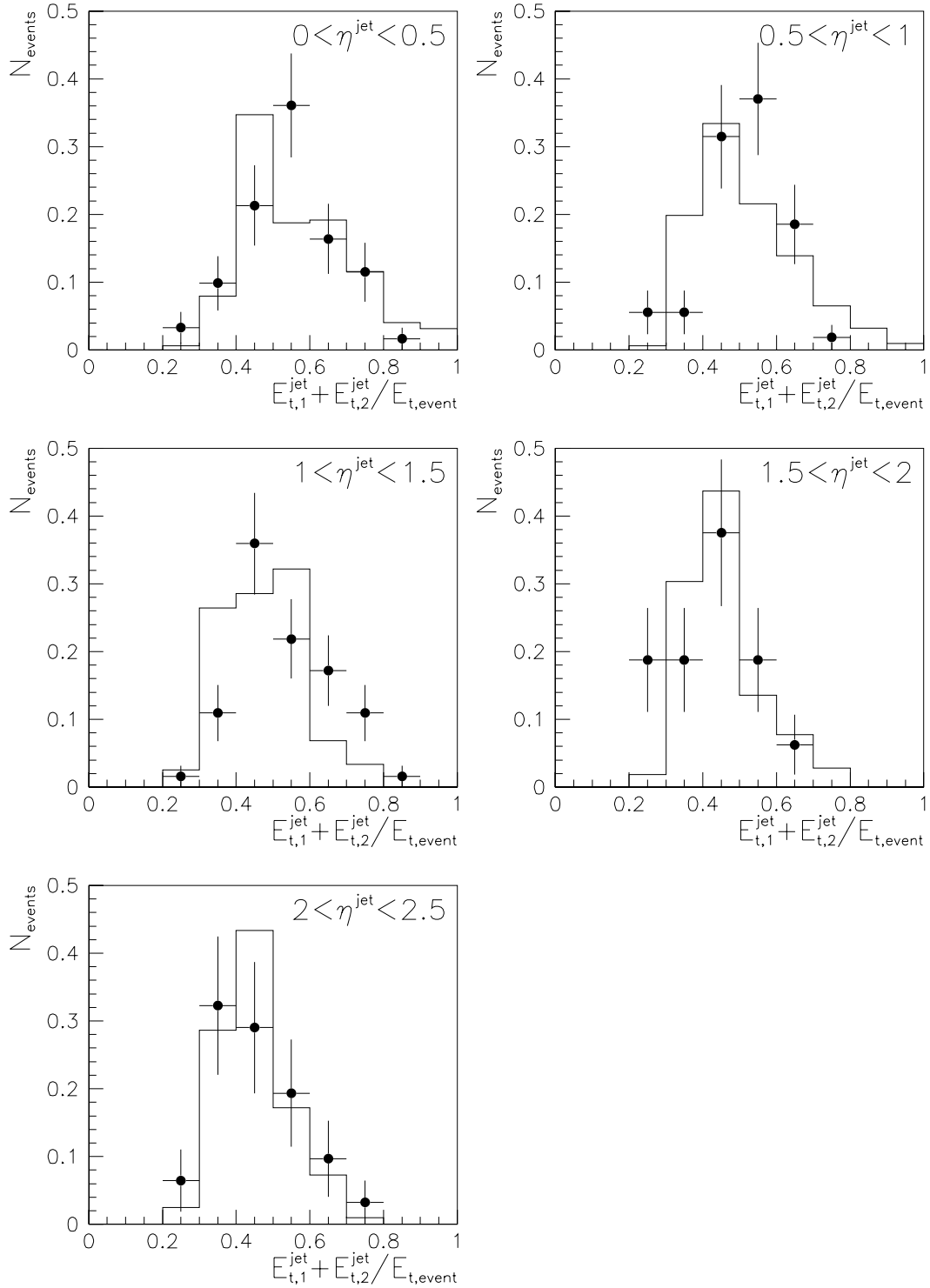
Figure 6.23: (E_{t,1}^{\text{jet}} + E_{t,2}^{\text{jet}}) / E_{t,\text{event}} -distribution as a function of \eta^{\text{jet}} for \delta_{\text{cut}} = 0.05 . Comparison of data (points) and MC (histogram; the MC is normalized to the integrated luminosity of the data sample). The MC sample used includes multiple interactions. The distributions are normalized to unit area.
