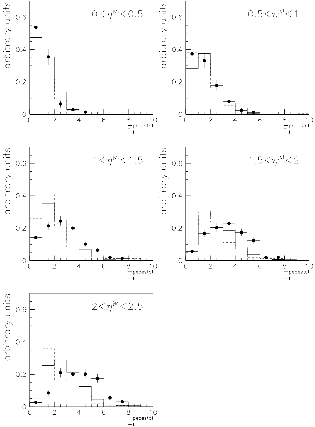
Figure 6.9: E_t^{\text{pedestal}} -distribution as a function of \eta^{\text{jet}} . Data (points) is compared with a Monte Carlo simulation that includes multiple interactions (full histogram) and a MC simulation without additional interactions (dashed histogram). The distributions are normalized to unit area.
