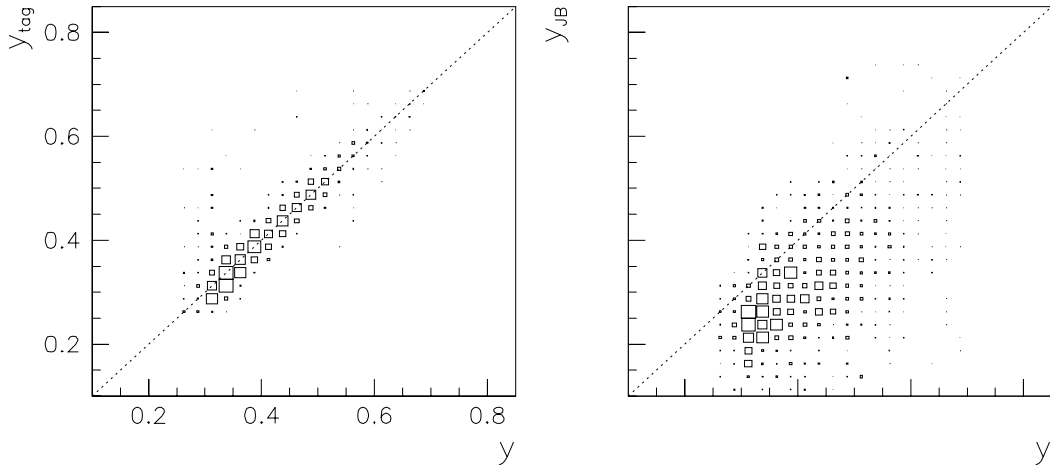
Figure 4.5: Correlation of true y with y_{\text{tag}} and y_{\text{JB}} , respectively.
