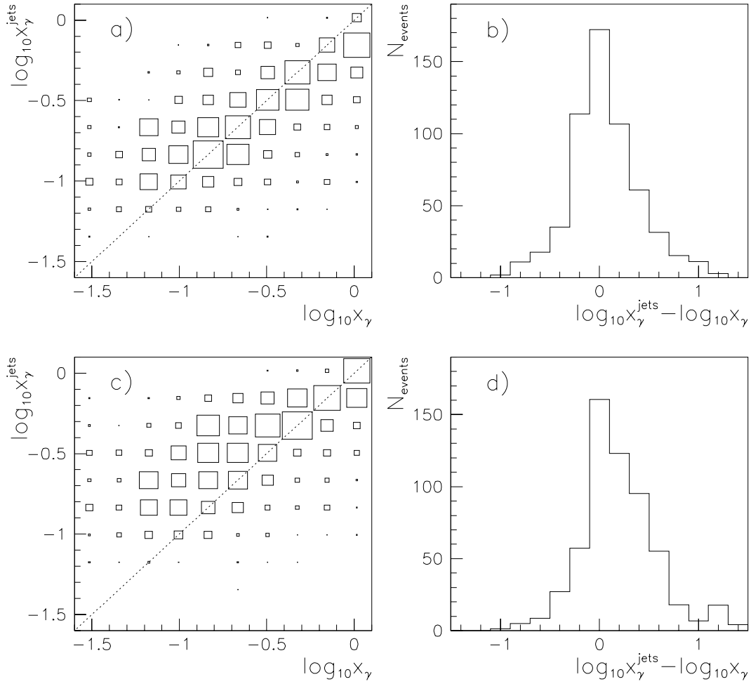
Figure 4.6: Correlation between x_{\gamma}^{\text{jets}} and true x_{\gamma} . For figures a) and b), y_{\text{tag}} is used for the determination of x_{\gamma}^{\text{jets}} whereas for figures c) and d) y_{\text{JB}} is used.
