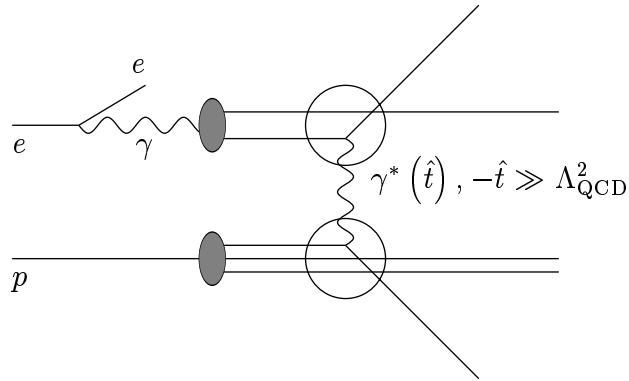
Figure 1.4: Hard scattering in photoproduction.
