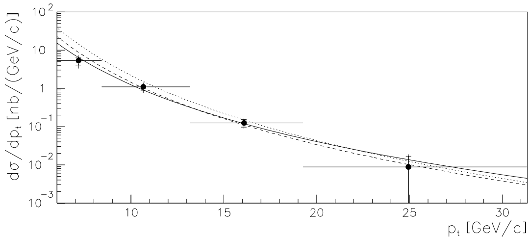
Figure 7.10: Inclusive parton cross-section d\sigma/dp_t in ep scattering versus the transverse momentum p_t for \sqrt{s_{ep}} = 296 GeV, Q^2 < 0.01 GeV 2 , 0.25 < y < 0.7 and 0 < \eta < 2.5 determined for the sub-jet sample. Inner error-bars show statistical errors, whereas outer error-bars are the (square root of the) quadratic sum of statistical and systematic errors, thereby neglecting the systematic error \sigma_{\text{others}} of 29.5%. The unfolding is performed by means of a Monte Carlo simulation which is based on leading order (partonic) matrix elements (see text). Comparison with theoretical predictions using the parton density function parametrizations of the photon by Glück, Reya and Vogt (GRV-LO, full line) and Abramowicz, Charchuła and Levy (LAC I, dashed line; LAC III, dotted line).
