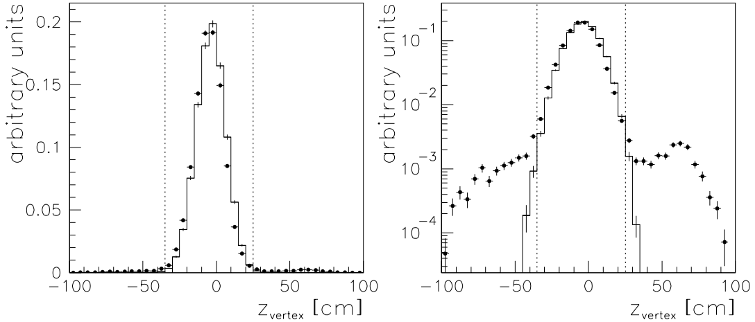
Figure 5.2: z -distribution (in linear and logarithmic scale) of the event-vertex for data (points) and MC (histogram). Data and MC are normalized to unit area. The dotted lines indicate the cut values.
