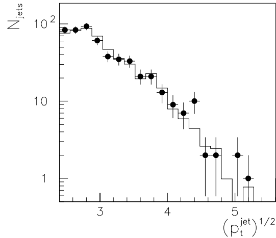
Figure 7.5: (p_t^{\text{jet}})^{1/2} -distribution. Comparison of the data distribution (points) with the reweighted Monte Carlo distribution (histogram). The MC is normalized to the integrated luminosity of the data sample. The final, pedestal subtracted samples are used.
