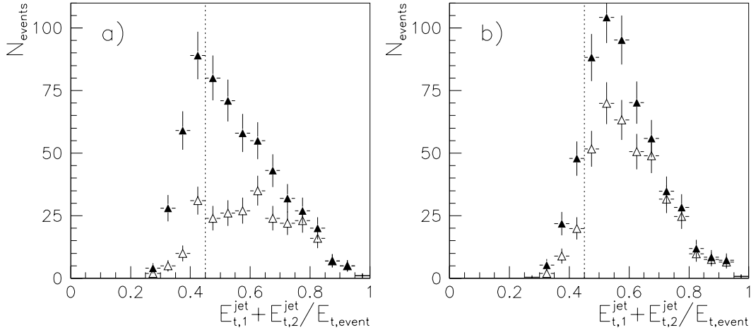
Figure 6.20: (E_{t,1}^{\text{jet}} + E_{t,2}^{\text{jet}})/E_{t,\text{event}} -distribution before ( \blacktriangle ) and after ( \triangle ) the pedestal subtraction. Shown are the distributions for the data sample (a)) and for the MC sample that includes multiple interactions (b)). The dotted lines indicate the cut at (E_{t,1}^{\text{jet}} + E_{t,2}^{\text{jet}})/E_{t,\text{event}} = 0.45 . Note that the jet energies used for the determination of (E_{t,1}^{\text{jet}} + E_{t,2}^{\text{jet}})/E_{t,\text{event}} are the uncorrected ones for the pedestal subtracted samples.
