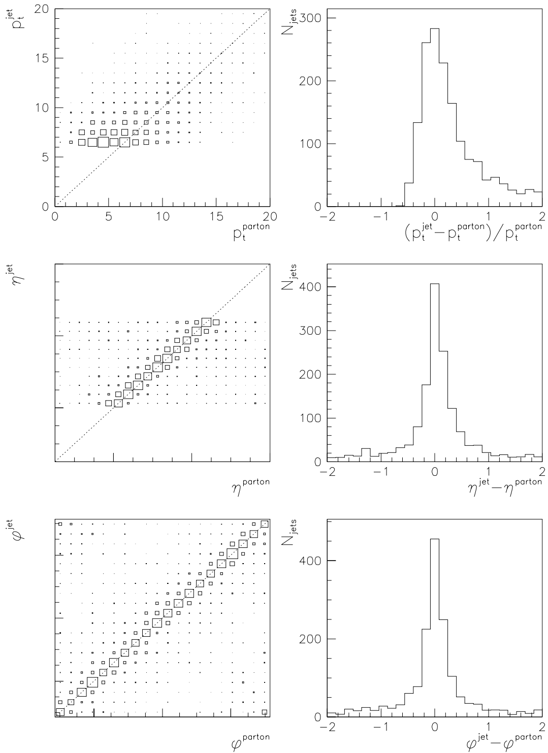
Figure 4.2: Jet parton correlation for p_t , \eta and \phi .
