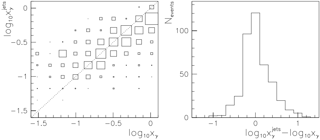
Figure 7.2: Correlation between x_\gamma^{\text{jets}} and x_\gamma .
