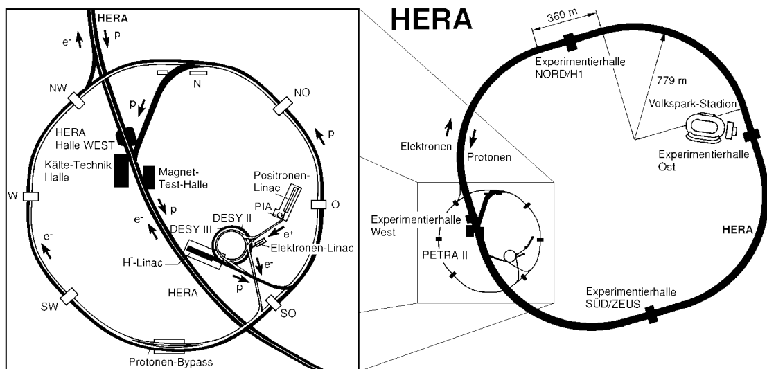
Figure 2.1: HERA and its pre-accelerators.
