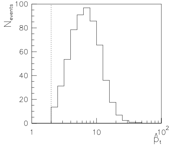
Figure 6.2: \hat{p}_t -distribution for the final MC sample (including multiple interactions). The cut on \hat{p}_t when generating the MC events was set to \hat{p}_{t,\text{min}} = 2 \text{ GeV}/c (dotted line).
