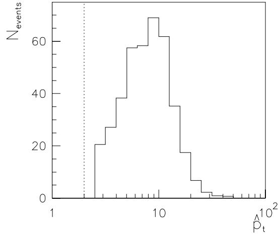
Figure 6.15: \hat{p}_t -distribution for the final, pedestal subtracted MC sample. The cut on \hat{p}_t when generating the MC events was set to \hat{p}_{t,\min} = 2 \text{ GeV}/c (dotted line).
