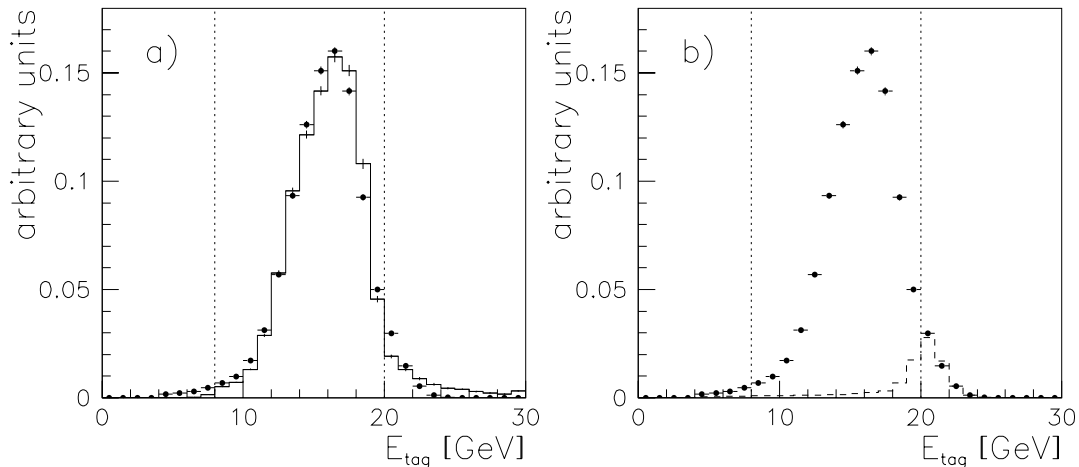
Figure 5.3: E_{\text{tag}} -distribution for data, MC and background events. In figure a), the E_{\text{tag}} -distribution (normalized to unit area) for data (points) and MC (histogram) is shown. Figure b) again shows the data distribution (points) together with the E_{\text{tag}} -distribution for the background events (dashed histogram). The background distribution is normalized such that the number of events above 20 GeV is equal for both distributions. The dotted lines indicate the cut values.
