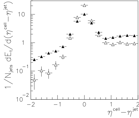
Figure 6.6: Jet-profile in \eta for the final data sample. Transverse energy flow (per jet) around the jet direction in a slice of |\varphi^{\text{cell}} - \varphi^{\text{jet}}| < 1 versus the distance in \eta from the jet axis. Jets are selected with 0 < \eta^{\text{jet}} < 1 and the profiles are given for x_{\gamma}^{\text{jets}} < 0.5 ( \blacktriangle ) and x_{\gamma}^{\text{jets}} > 0.7 ( \triangle ).
