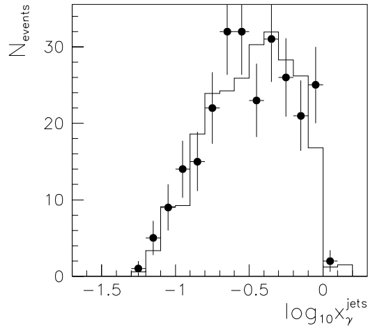
Figure 7.16: \log_{10}x_\gamma^{\text{jets}} -distribution. Comparison of the data distribution (points) with the reweighted Monte Carlo distribution (histogram). The MC is normalized to the integrated luminosity of the data sample. The final, pedestal subtracted samples are used.
