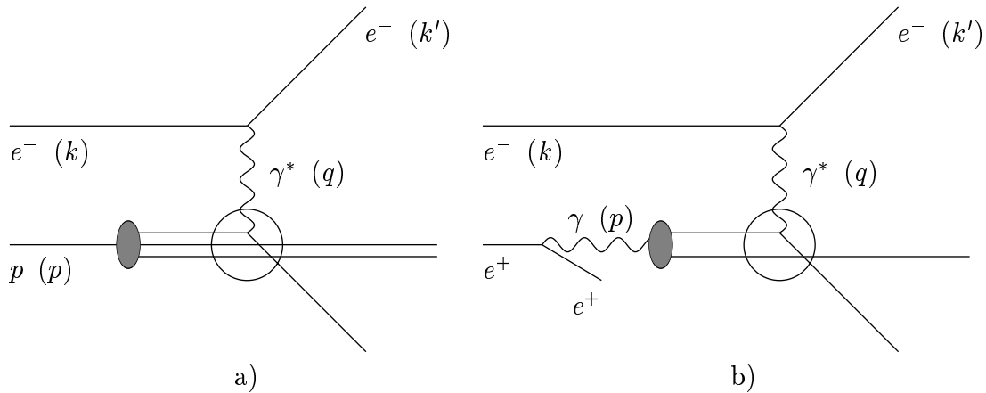
Figure 1.2: Diagrams describing deep inelastic scattering off a) a proton b) a quasi-real photon emitted from a positron.
