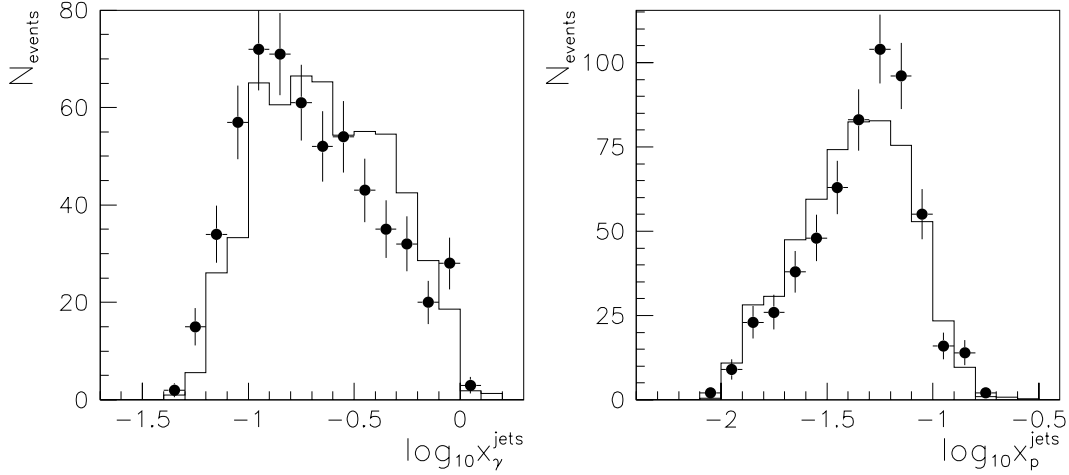
Figure 6.4: \log_{10}x_{\gamma}^{\text{jets}} - and \log_{10}x_p^{\text{jets}} -distribution for 2-jet events. Comparison of data (points) and MC (histogram; the MC is normalized to the integrated luminosity of the data sample). The MC sample (which includes multiple interactions) is based on the GRV-LO parton density function parametrizations for the photon and the proton.
