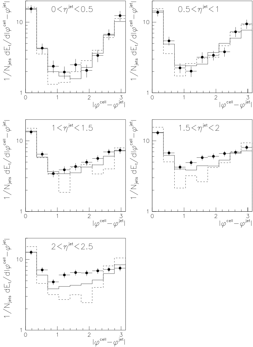
Figure 6.5: Jet-profiles in \varphi (see text) as a function of \eta^{\text{jet}} . Jets are selected with 6 \text{ GeV}/c < p_t^{\text{jet}} < 8 \text{ GeV}/c . Data (points) is compared with a Monte Carlo simulation that includes multiple interactions (full histogram) and a MC simulation without multiple interactions (dashed histogram).
