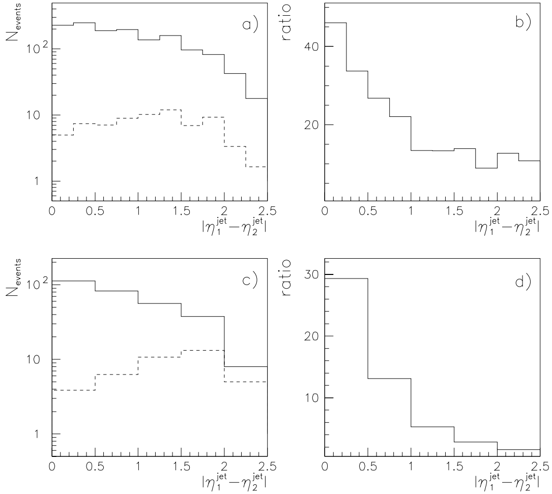
Figure 4.3: Pseudo-rapidity difference |\eta_1^{\text{jet}} - \eta_2^{\text{jet}}| . Events with no misidentified jets (full line) and events where one of the jets was matched with the photon remnant (dashed line) are shown for the entire x_\gamma -range (a,b)) and for x_\gamma < 0.1 (c,d)). Figures b) and d) show the ratio of the two contributions.
