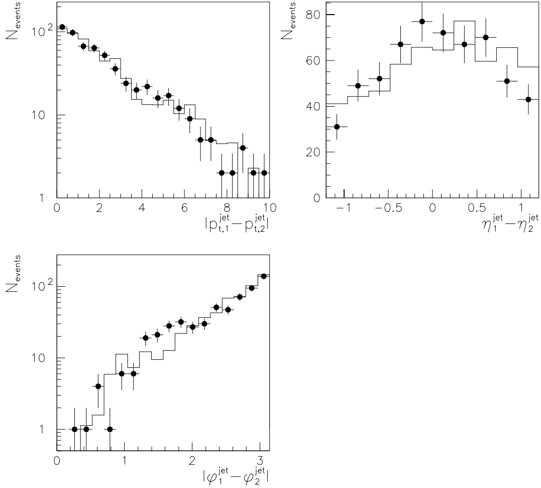
Figure 6.3: |p_{t,1}^{\text{jet}} - p_{t,2}^{\text{jet}}| , \eta_1^{\text{jet}} - \eta_2^{\text{jet}} and |\varphi_1^{\text{jet}} - \varphi_2^{\text{jet}}| distribution for 2-jet events. Comparison of data (points) and MC (histogram; the MC is normalized to the integrated luminosity of the data sample). The MC sample used includes multiple interactions.
