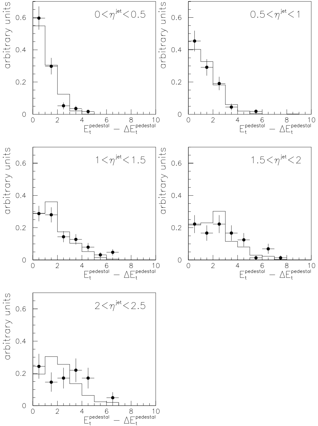
Figure 6.14: E_t^{\text{pedestal}} - \Delta E_t^{\text{pedestal}} distribution as a function of \eta^{\text{jet}} . Comparison of data (points) and Monte Carlo simulation (full histogram). The distributions are normalized to unit area.
