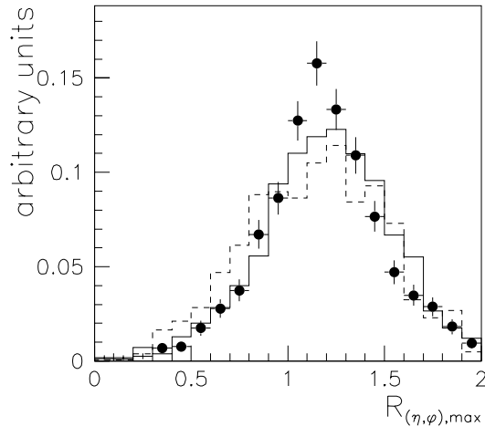
Figure 6.11: R_{(\eta,\varphi),\text{max}} -distribution for the final data (points) and MC samples (full histogram: including multiple interactions; dashed histogram: no additional interactions). R_{(\eta,\varphi),\text{max}} is given by the cluster assigned to the jet by the k_{\perp} -algorithm which has the largest distance R_{(\eta,\varphi)} = \sqrt{(\eta^{\text{cluster}} - \eta^{\text{jet}})^2 + (\varphi^{\text{cluster}} - \varphi^{\text{jet}})^2} from the jet axis. To account for the fact that the reconstruction code may produce clusters of vanishing energy ( e.g. due to noise suppression procedures), a minimal energy of E_{\text{cluster},\text{min}} = 50 \text{ MeV} is asked for every cluster.
