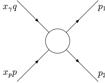
Figure 1.7: Hard parton parton scattering.
