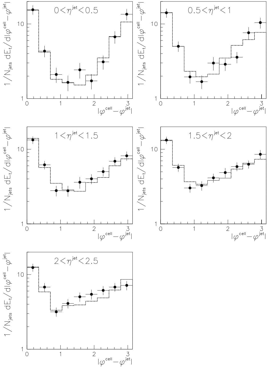
Figure 6.18: Jet-profiles in \varphi as a function of \eta^{\text{jet}} after the cut on (E_{t,1}^{\text{jet}} + E_{t,2}^{\text{jet}})/E_{t,\text{event}} . Jets are selected with 6 \text{ GeV}/c < p_t^{\text{jet}} < 8 \text{ GeV}/c . Data (points) is compared with a Monte Carlo simulation that includes multiple interactions (full histogram).
