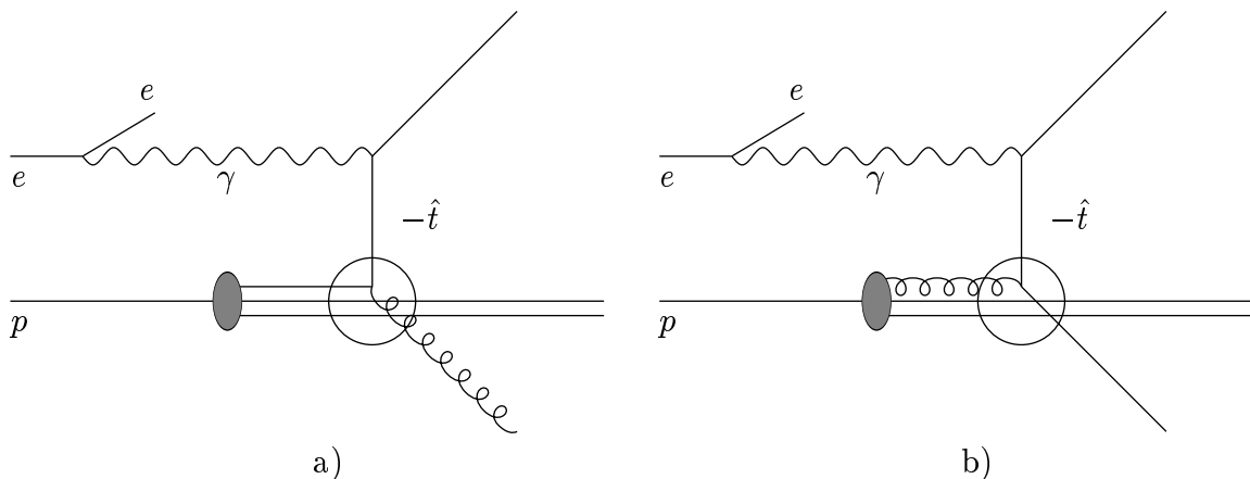
Figure 1.5: Direct processes (LO QCD) in photon proton scattering: a) QCD Compton scattering \gamma q \rightarrow gq , b) photon gluon fusion \gamma g \rightarrow q\bar{q} .
