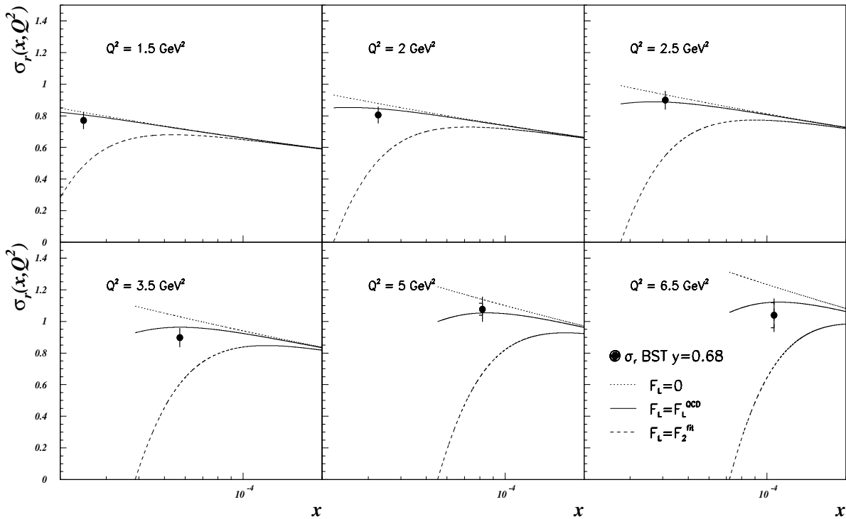
Figure 6.18: Reduced DIS cross section for y = 0.68 presented in six Q^2 bins. The inner error bars denote the statistical uncertainty and the full error bars represent the systematic and statistical uncertainties added in quadrature. Also shown are the curves corresponding to different assumptions on the structure function F_L .
