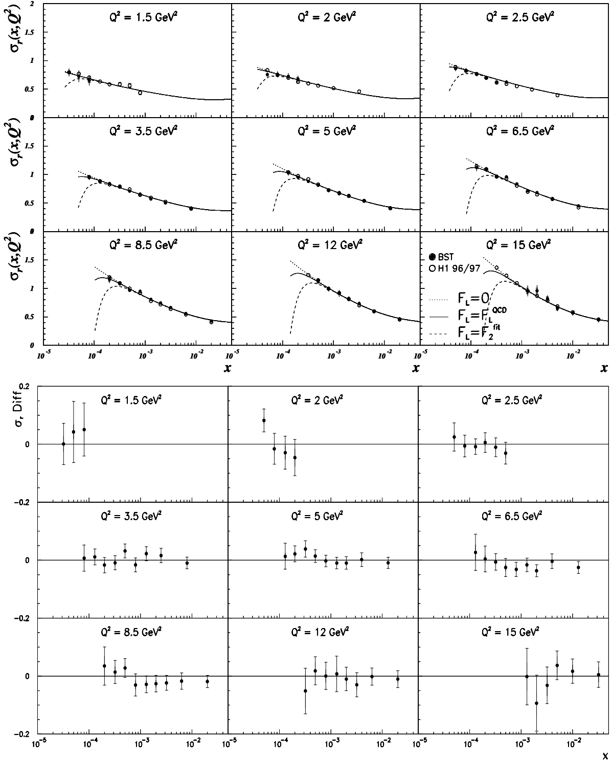
Figure 6.17: Top: Reduced DIS cross section ( \sigma_r = \sigma/\kappa ) presented for y < 0.6 as a function of x in different Q^2 bins. The results obtained in this BST analysis are compared with the \sigma_r data measured by H1. The inner error bars denote, where visible, the statistical uncertainty and the full error bars represent the statistical and systematic uncertainties added in quadrature. Also shown are the curves corresponding to NLO QCD predictions for the reduced cross section with different assumptions on the structure function F_L . Bottom: Difference between these two data on reduced DIS cross section. The error bars represent the statistical and the systematic uncertainties of the presented analysis added in quadrature.
