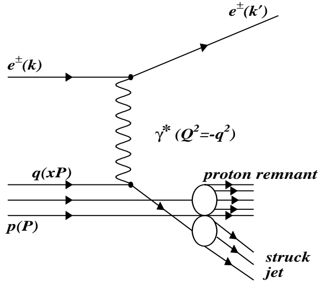
Figure 2.3: Schematic representation of deep inelastic ep scattering in the Quark Parton Model. The virtual photon interacts with a free, point-like charged parton carrying a fraction xP of the proton momentum. The interaction proceeds with hadronization resulting in a “proton remnant” jet and a “struck jet” emitted along the direction of the struck quark.
