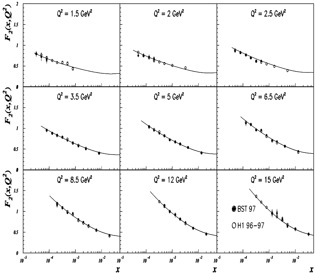
Figure 6.19: The proton structure function F_2 presented as a function of x in different Q^2 bins. The result of the analysis (closed circles) is compared with standard H1 analysis (open circles) based on the data collected in the years 1996 and 1997 [71]. Where visible, the inner error bars denote the statistical uncertainty and the full error bars represent the systematic and the statistical uncertainties added in quadrature.
