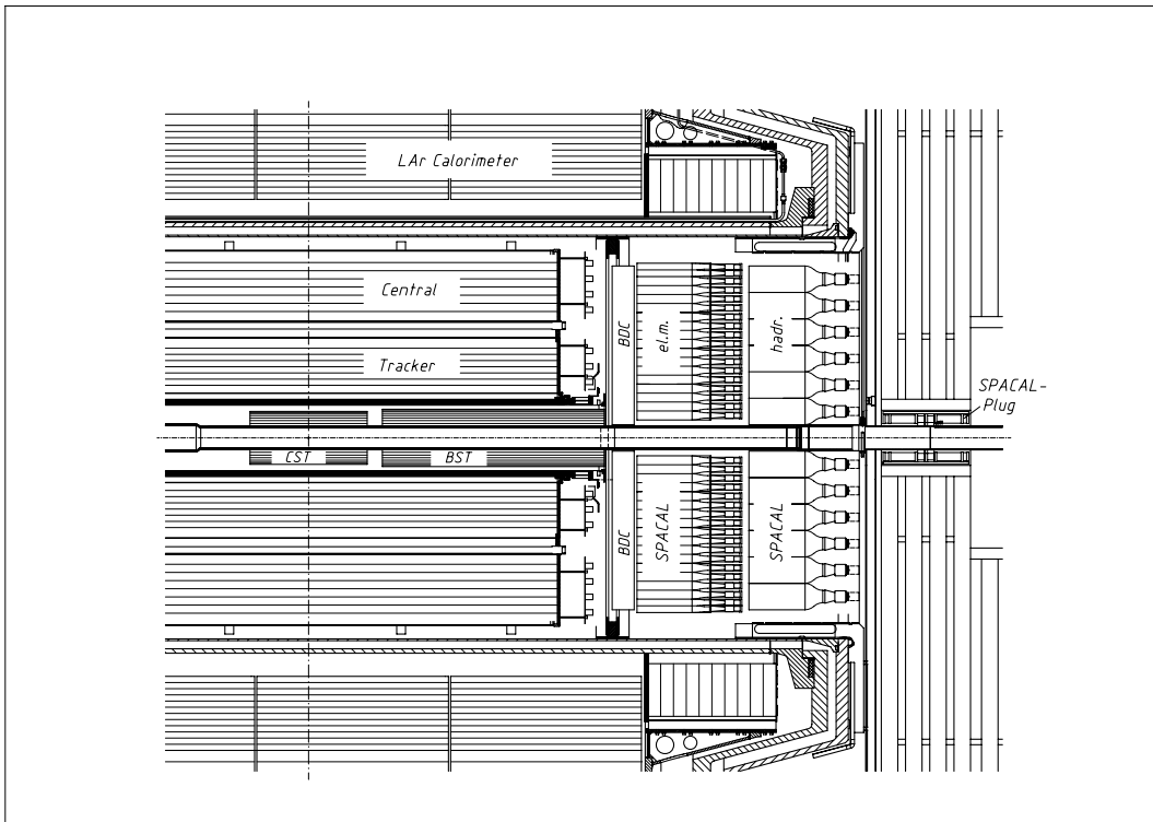
Figure 3.5: Schematic view of the backward part of the H1 detector.
