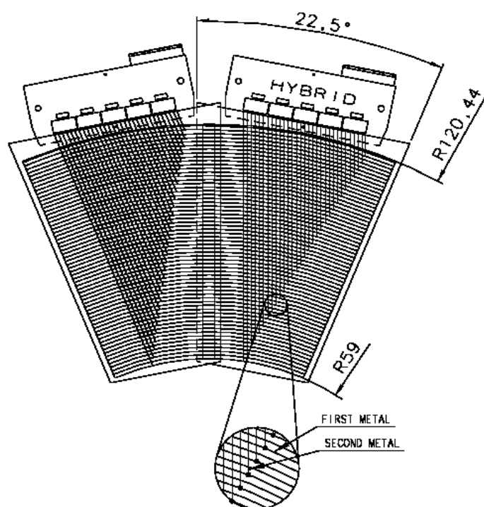
Figure 4.5: Schematic view of two adjacent BST sensors.
