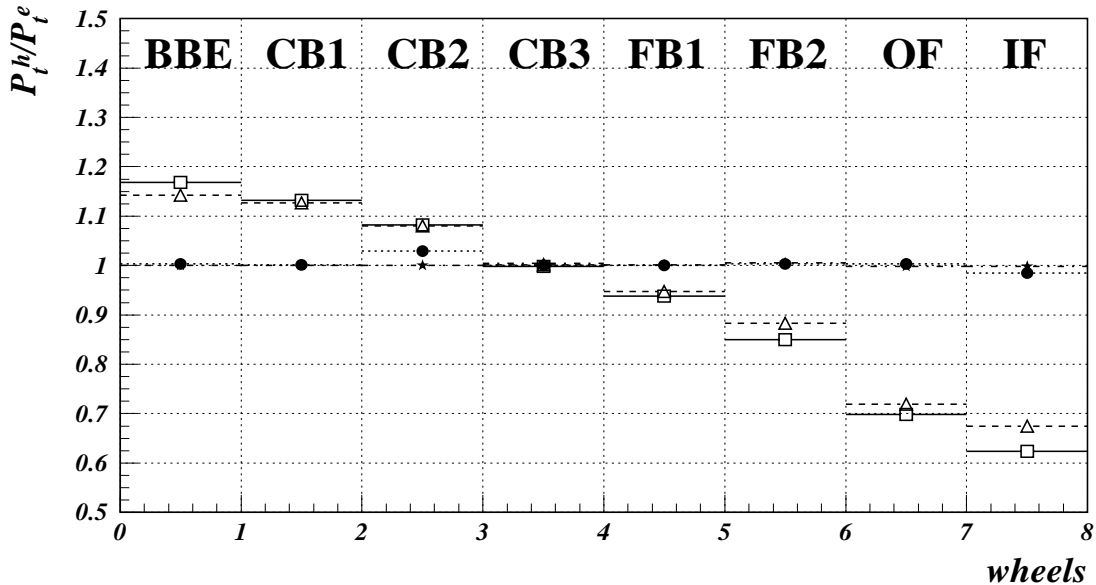
Figure 5.7: Comparison of the mean values of the P_t balance obtained from Gaussian fits performed to the ratio P_t^h/P_t^e for 8 wheels of the LAr calorimeter. The open boxes (triangles) represent the situation for data (Monte Carlo) before calibration and the closed boxes (stars) after 8 iterations.
