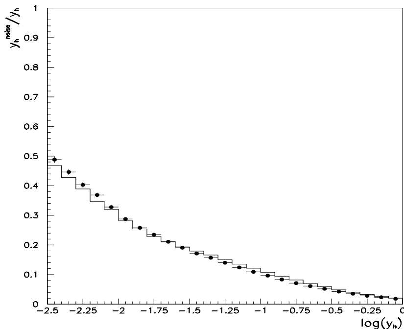
Figure 5.2: Contribution of the electronic noise of the LAr calorimeter to the reconstructed y_h as a function of y_h . Closed points present data and the histogram illustrates the Monte Carlo simulation.
