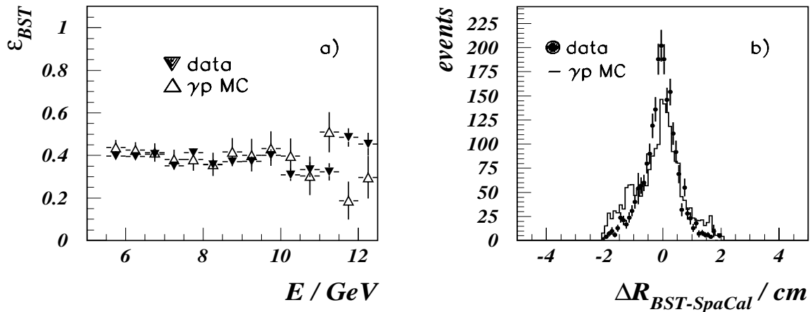
Figure 6.12: a) BST validation efficiency for the photoproduction background. The inefficiency represents the rejection power. Photoproduction background is reduced by a factor of about 2.5 in addition to the conventional DIS selection criteria. b) Matching between BST and SpaCal shown on the SpaCal plane. Poor agreement between photoproduction data and simulation made to open the matching criteria up to 2 cm to avoid possible bias in the cross section measurement.
