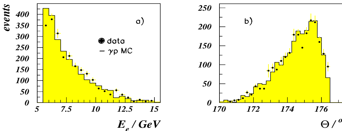
Figure 6.13: Energy (a) and polar angle (b) distributions for the tagged photoproduction events measured with the SpaCal and the BST, respectively, (closed circles), compared with the photoproduction simulation (histogram).
