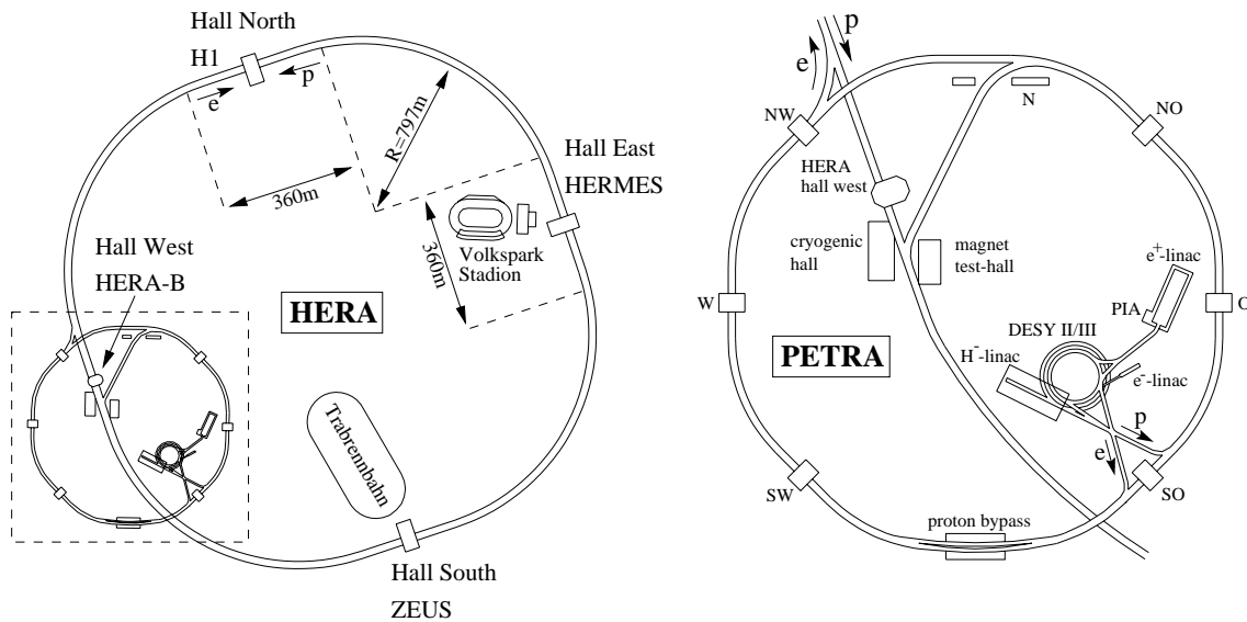
Figure 3.1: Schematic view of the ep storage ring HERA (left) together with the major experiments. The right figure presents a zoomed view of the HERA preaccelerator chain.
