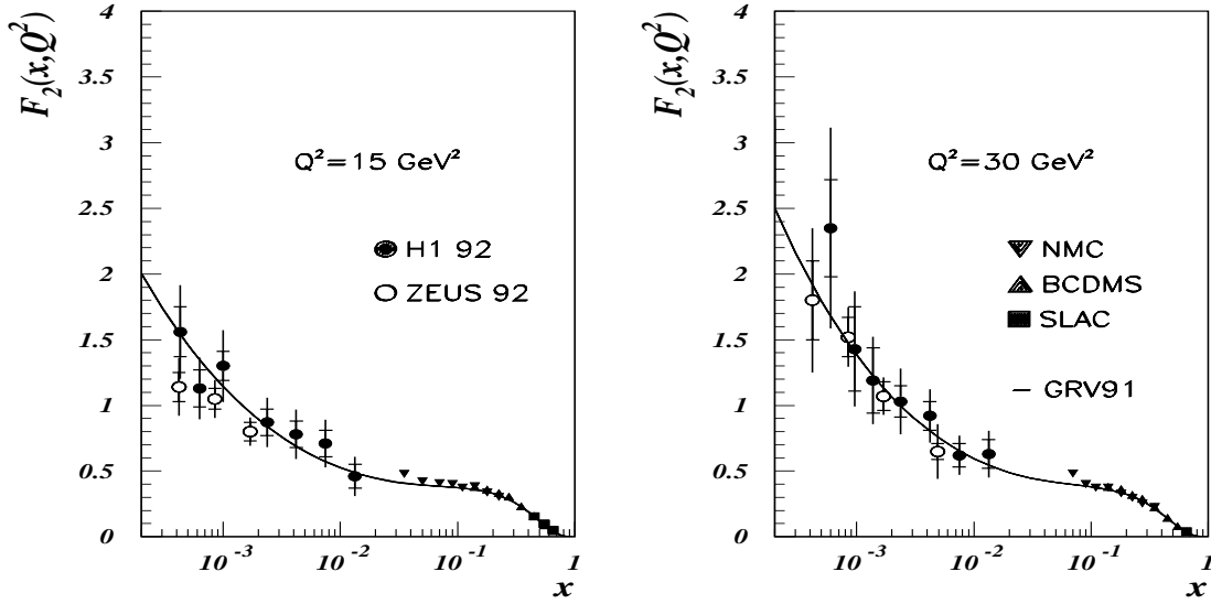
Figure 2.1: Measurements of the proton structure function F_2(x, Q^2) by the fixed target experiments SLAC, NMC and BCDMS and their extension towards low x represented by the first HERA data on F_2 . The curve represents the expectation of this rising behavior by GRV'91 [21].
