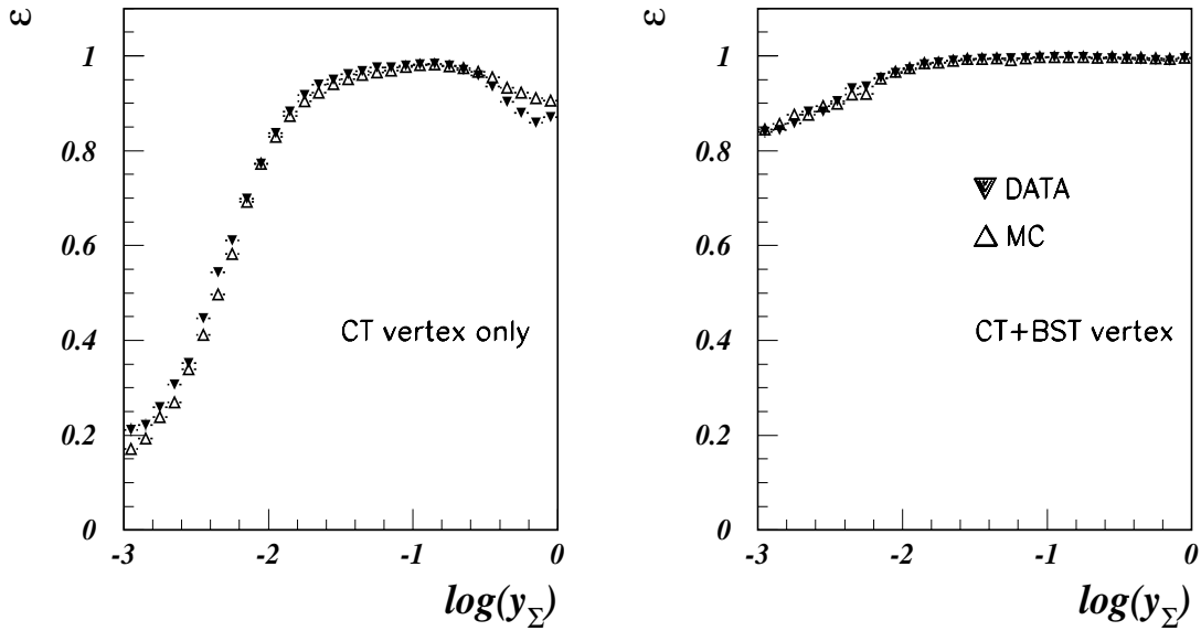
Figure 6.2: Vertex reconstruction efficiency as a function of y_{\Sigma} within the BST acceptance. The left picture represents the situation where only the central tracker vertices are used. The right picture is based on the reconstruction of the event vertex supplemented by the measurement of the scattered electron with the BST.
