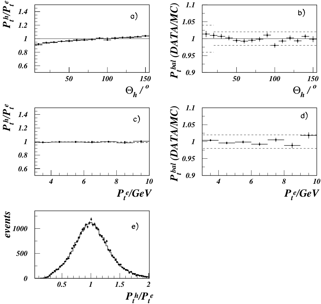
Figure 5.8: Control plots for the LAr calibration with the iterative method. Mean values of the P_t balance as a function of \theta_h (a) and P_t^e (c) for data (closed circles) and Monte Carlo (closed triangles). The corresponding ratios of the mean values between data and Monte Carlo are presented in figures b) and d). Dashed lines in figure b) represent the suggested systematical uncertainty of 2% for backward and central parts of the LAr calorimeter and of 4% for the forward one. The dashed lines in figure d) show that the data to Monte Carlo ratio of P_t balance mean values are well within 2% variations independently on the transverse momentum of the final state electron. Figure e) represents general shape of the P_t balance which is very good described by Monte Carlo simulation and both distributions are peaked at unity by construction.
