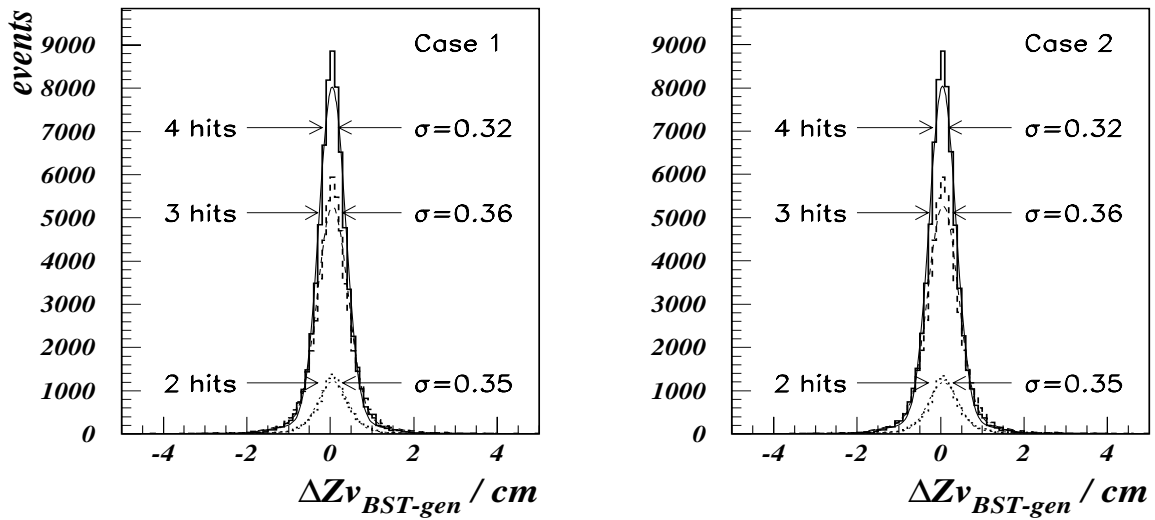
Figure A.6: Comparison of the z -vertex reconstruction performed within the corridor (left figure) and semi-combinatoric (right figure) approaches. The comparison is shown for 2, 3 and 4 BST hits defining the electron track reconstruction.
