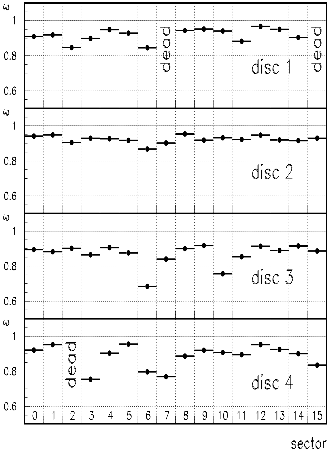
Figure 4.11: The internal efficiencies of the BST detectors for the special low Q^2 run taken in October 1997.
