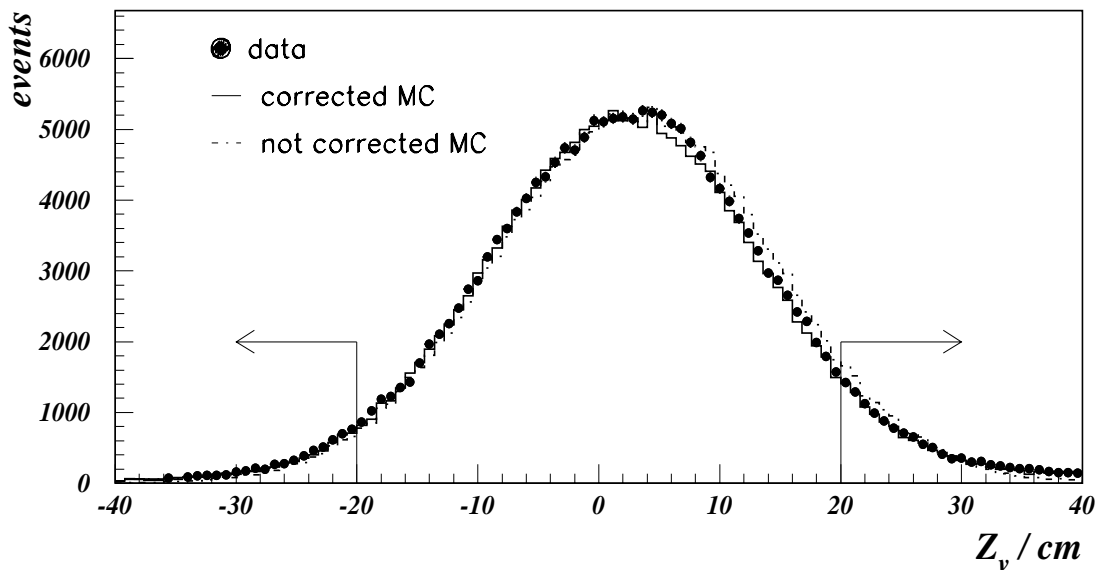
Figure 6.10: Distribution of the z -position of the interaction vertex in the data (closed circles) and in the z_v -reweighted Monte Carlo simulation (solid line). The hatched-dotted line represents the z -vertex distribution of the original Monte Carlo simulation. Also shown is the z -vertex cut when events outside \pm 20 cm are rejected.
