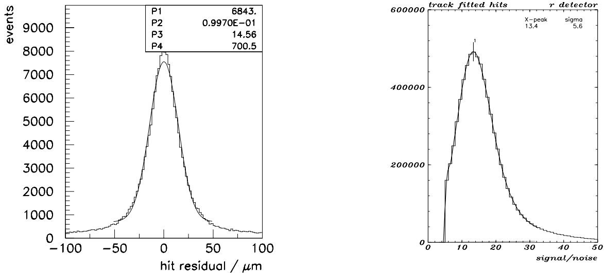
Figure 4.10: Left: Residual distribution of the BST. Right: Signal to noise ratio of the 64 detectors constituting the BST. A cut S/N > 5 has been applied during offline data processing.
