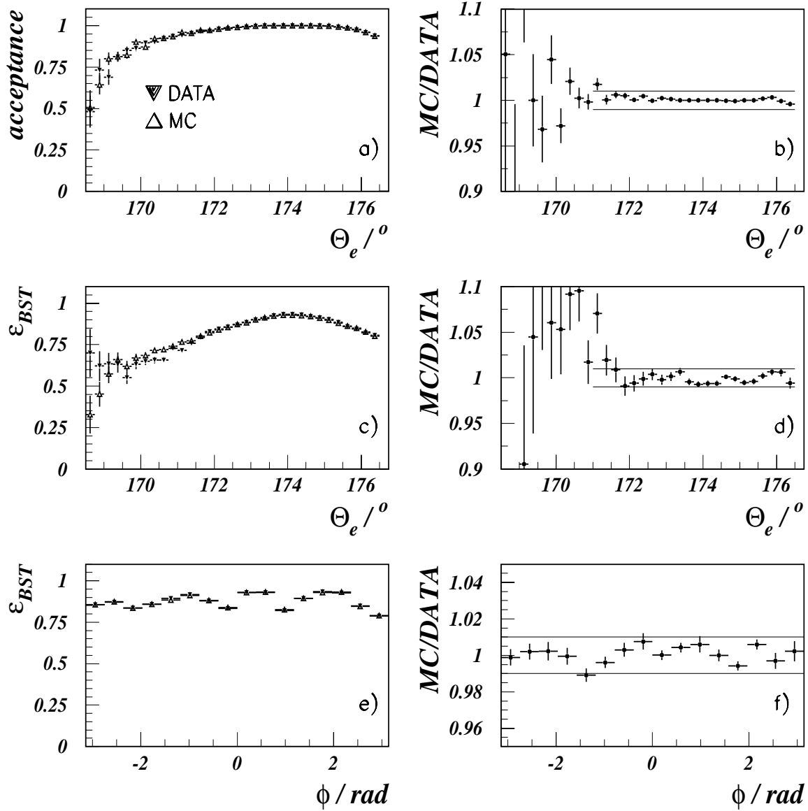
Figure 6.8: a) BST acceptance as a function of the polar angle and b) the corresponding ratio between simulation and data. c) BST efficiency within the acceptance as a function of the polar angle. The corresponding ratio between simulation and data is shown in d). e) BST efficiency within the acceptance as a function of the azimuthal angle. The corresponding ratio between simulation and data is shown in f). The 16 \phi bins correspond to the 16 fold azimuthal subdivision of the detector.
