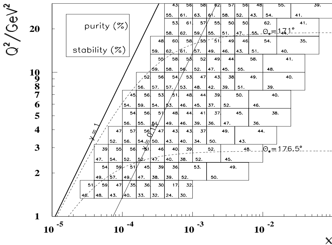
Figure 6.3: The values of purity and stability for different bins of the (x, Q^2) kinematic plane. The picture on the top (bottom) stands for electron ( \Sigma method), respectively. The solid lines show the constant inelasticity. For y > 0.15 ( y < 0.15 ) the electron ( \Sigma ) method has been used. Also shown are the lines of constant polar angle of the scattered electron illustrating the BST acceptance.
