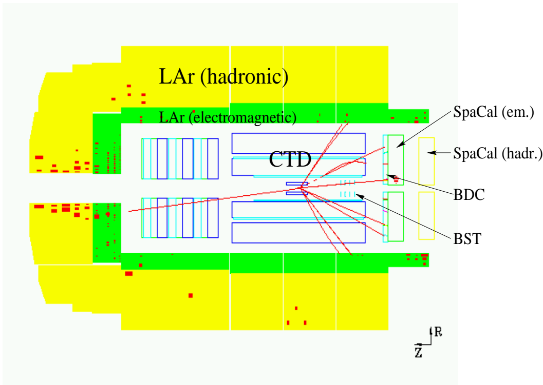
Figure 4.1: R - Z view of the H1 detector with a typical of a DIS event with the scattered electron measured with the BST.
