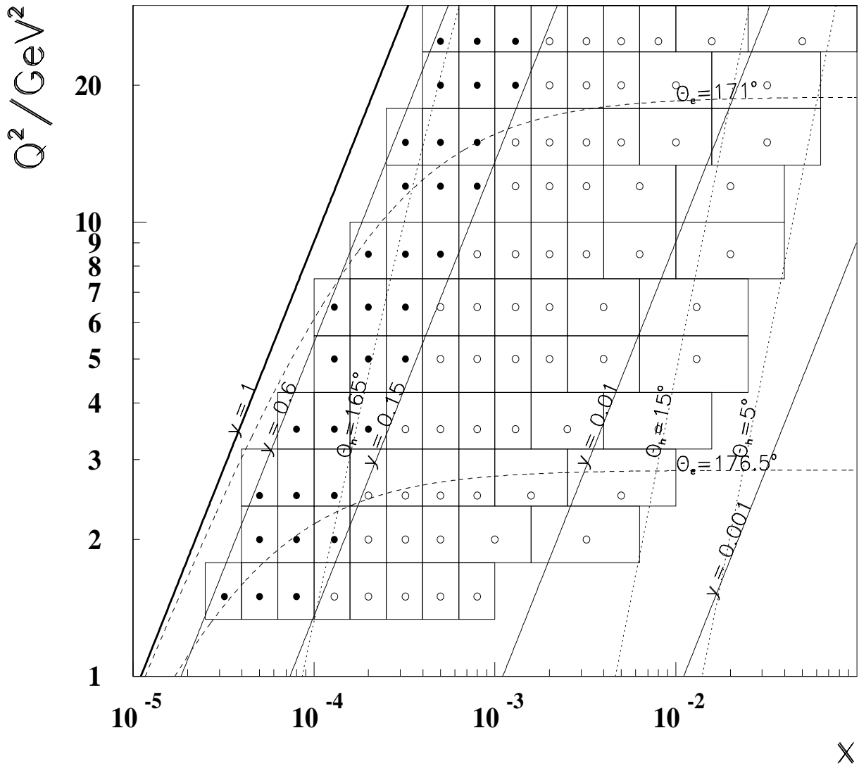
Figure 6.1: Kinematic plane of x and Q^2 . The grid represents the (x, Q^2) binning used in the analysis for y < 0.6 . The size of the bins is adapted to the resolution of the kinematic variables (see text). Closed (open) points indicate the bins where the electron ( \Sigma method) is used to measure the cross section, respectively. The dashed curves of constant polar angle \theta_e of the scattered electron denote the angular acceptance limits of the BST, whereas the dotted curves represent the approximate angular acceptance of the CJC at constant jet angles \theta_h = 165^\circ and \theta_h = 15^\circ . The dotted curve at \theta_h = 5^\circ depicts the lowermost acceptance of the LAr calorimeter. Also shown are lines of constant inelasticity y .
