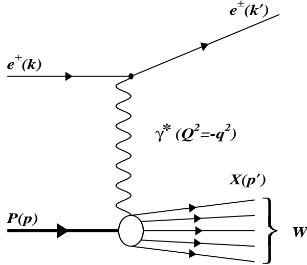
Figure 2.2: Schematic representation of inclusive electron proton scattering e^\pm p \rightarrow e^\pm X at low Q^2 with the single photon exchange approximation. The four-momenta of the incoming and scattered lepton are k and k' , respectively. The four-momentum of the incident proton is p and p' denotes the four-momentum of the hadronic final state X with the invariant mass W .
