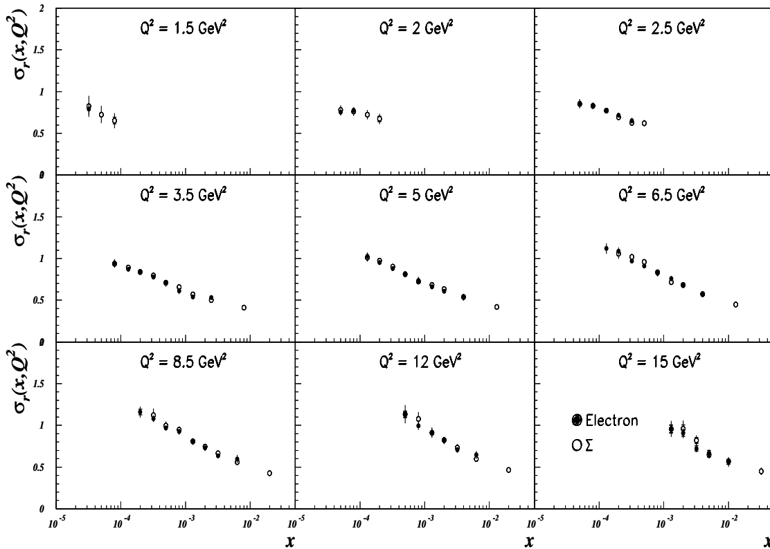
Figure 6.16: Reduced DIS cross section measured with the electron (closed circles) and \Sigma (open circles) methods shown for y < 0.6 . The inner error bars denote the statistical uncertainty, the full error bars correspond to the systematic and the statistical errors added in quadrature.
