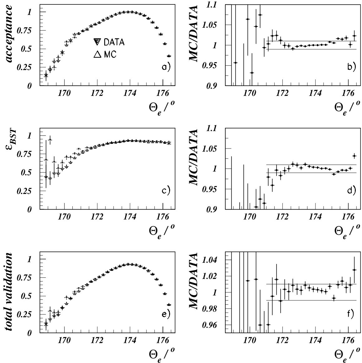
Figure 6.9: a) BST acceptance with R_{max} = 11.5 cm and R_{min} = 6.5 cm (see text) as a function of the polar angle and b) the corresponding ratio between simulation and data. c) BST efficiency within the acceptance as a function of the polar angle. The corresponding ratio between simulation and data is shown in d). e) Superposition of the BST acceptance and efficiency which represents the total validation as a function of polar angle. The corresponding ratio between simulation and data is shown in f). All quantities are described within 1% of systematic uncertainty apart from the edges of the BST acceptance.
