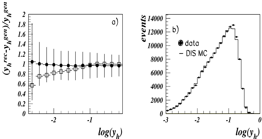
Figure 5.6: a) Comparison of y_h reconstruction before (open boxes) and after (closed circles) LAr calibration. The error bars represent the mean values and their statistical error (spread) obtained from Gaussian fits performed to the quantity (y_h - y_{gen})/y_{gen} in slices of y_{gen} for uncalibrated (calibrated) case. The y_h resolution is seen to degrade to unacceptably large values at \log(y_h) < -2.5 with a fixed \log(y_h) bin width. b) y_h distribution for data (closed points) and Monte Carlo (histogram) after performing the calibration of the LAr hadronic energy scale and imposing the P_t balance cut (see in the text).
