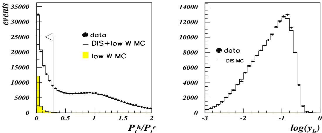
Figure 6.7: Left: P_t balance distribution for energies E'_e > 20 GeV. Closed points represent data. The shaded histogram illustrates DIS events with W_{gen} < 5 GeV simulated with the HERWIG generator. The open histogram represents the sum of two simulated event samples with W_{gen} < 5 GeV (HERWIG) and W_{gen} > 5 GeV (DJANGO). The peak at zero corresponds to DIS events with a large fraction of hadronic final state particles scattered below the forward modules of the LAr calorimeter. Events with P_t^h/P_t^e < 0.3 for E'_e > 24 GeV were rejected (see text). Right: The y_h distribution for energies E'_e > 20 GeV with applied P_t balance cut. Closed points represent data. The histogram illustrates the DIS Monte Carlo simulation. Less than 1% of the low W events pass the P_t balance cut, therefore, they were not added to the final Monte Carlo simulation.
