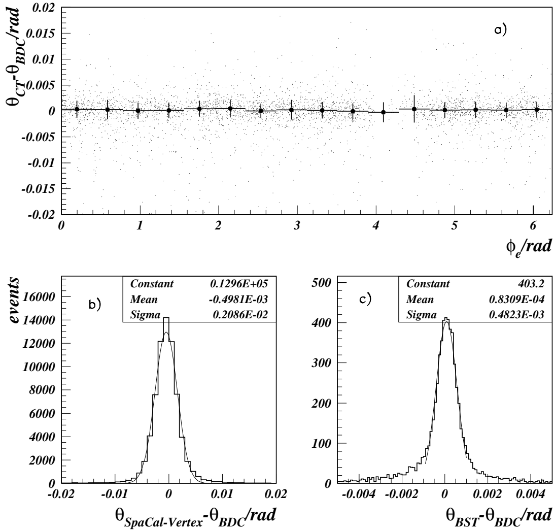
Figure 4.16: a) Difference of the scattered electron polar angle measured with the central trackers and with the BDC as a function of the azimuthal angle \phi_e after alignment. Solid circles with error bars on plot a) represent the mean values \Delta\theta with their statistical errors of the Gaussian fit performed in \phi_e slices. Matching of the scattered electron polar angles measured with the SpaCal-vertex combination and with the BDC is visible in Fig. b). Fig. c) illustrates the matching of the scattered electron angle measurements with the BST and the BDC for the case when a track in the BST was reconstructed from four hits. All three plots were made when no showering occurred in front of the BDC.
