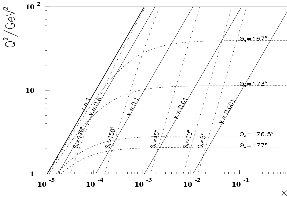
Figure 4.2: Kinematic range covered by the BST. The dashed lines of constant polar angle \theta_e represent the BST acceptance. The outer (inner) lines mark the “2-out-of-4” (“4-out-of-4”) region which is accessed with two or four BST planes out of the 4 existing. The dotted curves correspond to constant jet angles \theta_h . Also shown are lines of constant inelasticity y .
