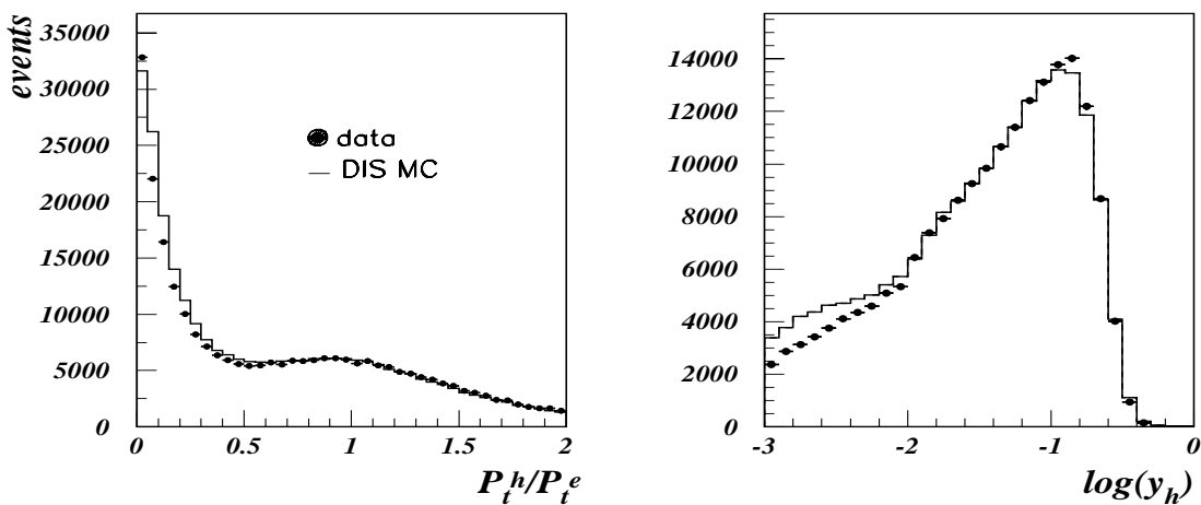
Figure 6.6: Left: P_t balance distribution for energies E'_e > 20 GeV. Right: The y_h distribution for E'_e > 20 . Closed points represent data. The histogram represents the simulated event sample with double counting of events with 5 < W_{gen} < 10 GeV (see text).
