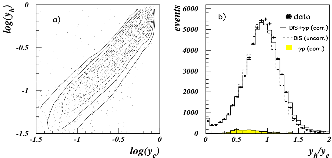
Figure 5.1: Contour lines in figure a) illustrate the correlation between y_h and y_e plotted for data. Figure b) shows the ratio y_h/y_e for data (closed circles) and for Monte Carlo simulation before (dashed line) and after (solid line) applying a correction factor of 1.06 (see text).
