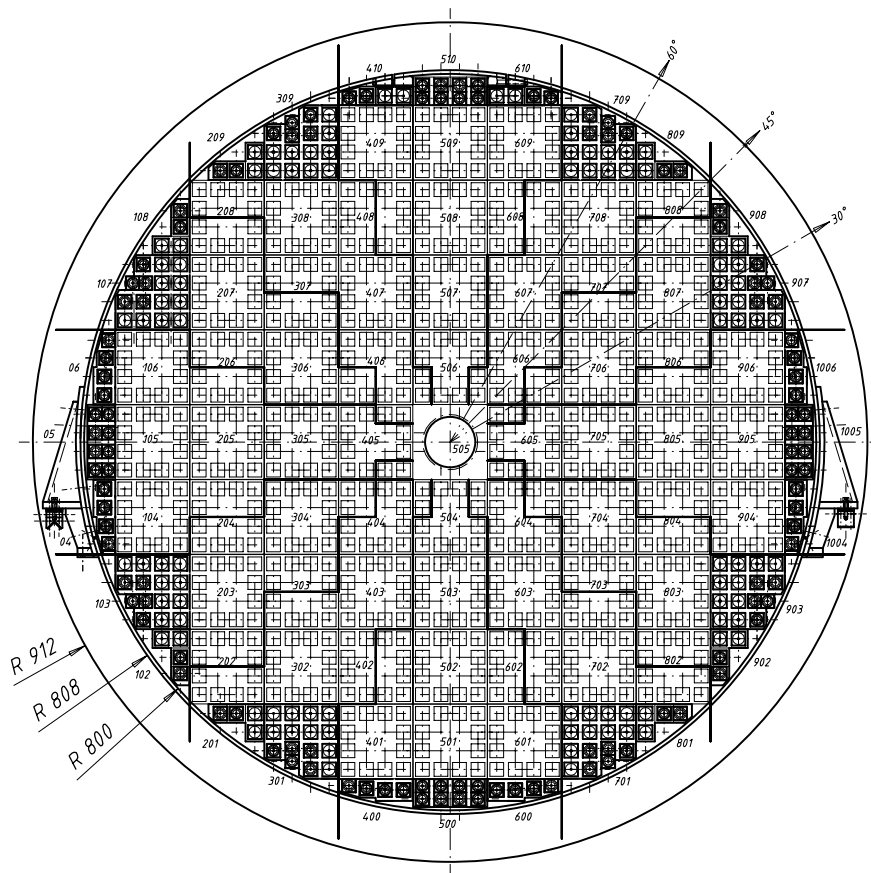
Figure 3.6: Schematic transverse view of the SpaCal electromagnetic calorimeter.
