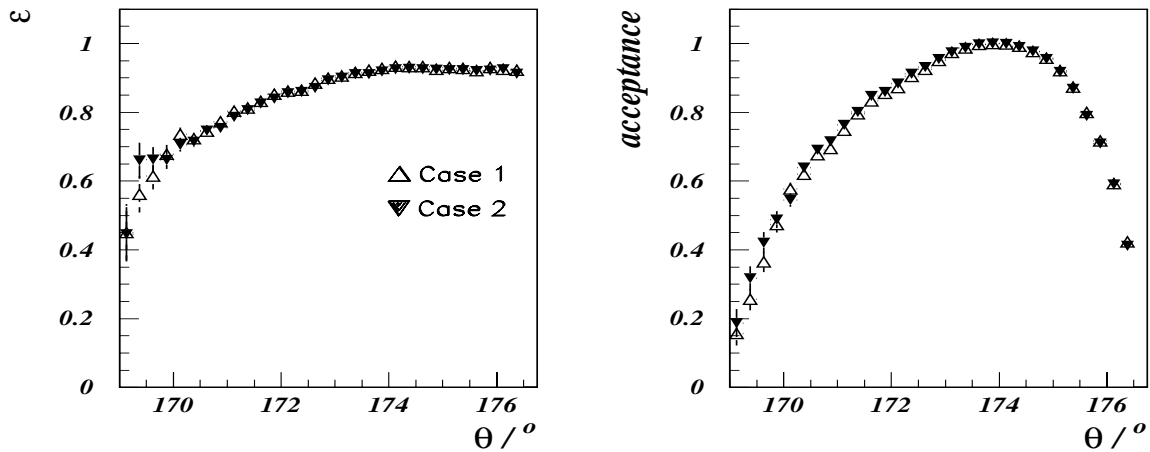
Figure A.4: Comparison of the BST efficiency (left figure) and acceptance (right figure) between the two approaches used in the electron finding procedure.
