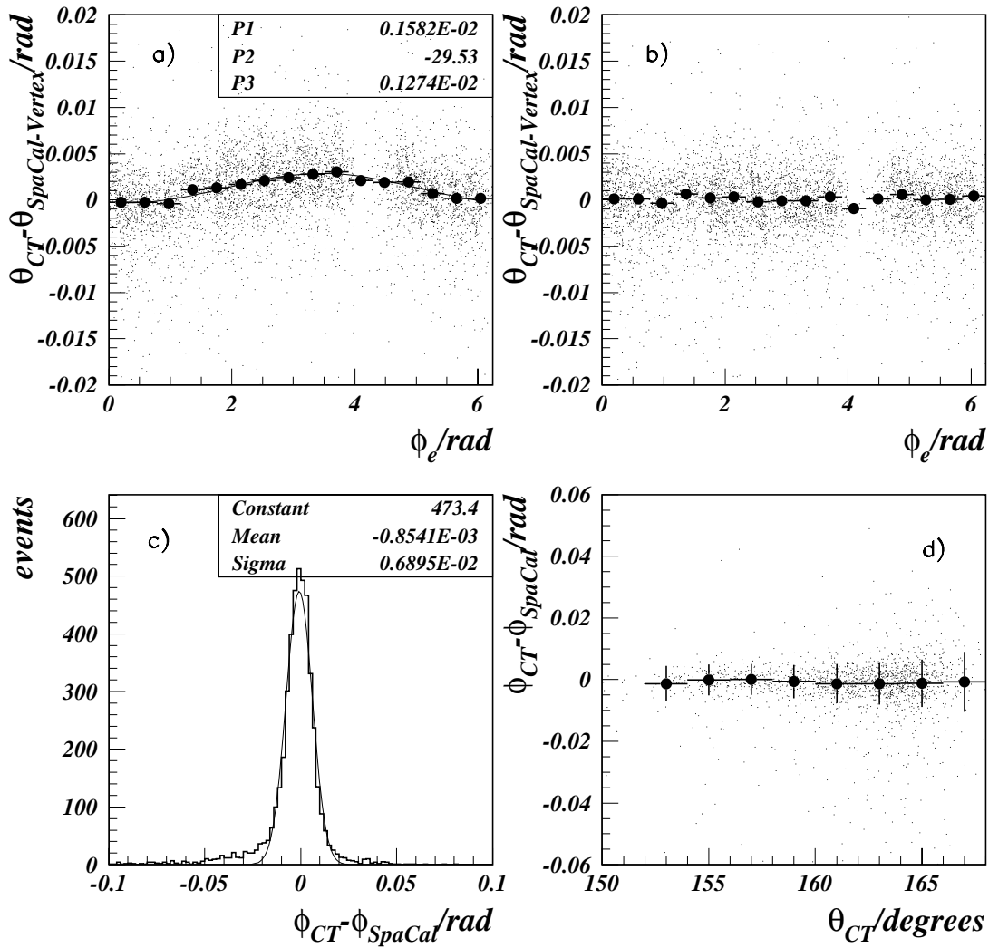
Figure 4.15: Difference of the scattered electron polar angle measured with the central trackers and SpaCal-vertex combination as a function of azimuthal angle \phi_e measured by SpaCal before alignment (a) and after alignment (b). Solid circles with error bars represent the mean values and their statistical errors of Gaussian fits performed in \phi_e slices. Plot c) displays the matching between the azimuthal angle \phi_e measured by central trackers and the backward electromagnetic calorimeter after alignment. Its dependence on the polar angle \theta_e is presented in plot d) where the solid circles with error bars represent the mean values and the spread of Gaussian fits performed in \theta_e slices.
