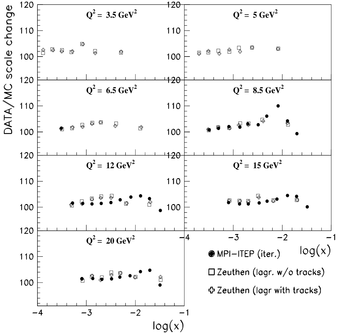
Figure 5.9: Comparison of the relative change of the hadronic energy scale (see Eq. 5.6) between three different calibrations as a function of \log(x) represented in seven low Q^2 bins. The variations of the points are normally within \pm 2\% ( 4\% ) from the average change of the hadronic energy scale for low and middle (high) x . Note that at low y , binning in x is different for two analyses.
