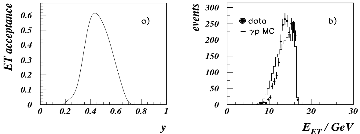
Figure 6.11: a) Acceptance of the electron tagger as a function of inelasticity. b) Energy distribution of the electrons measured with the electron tagger after all \gamma p selection cuts being applied (see text).
