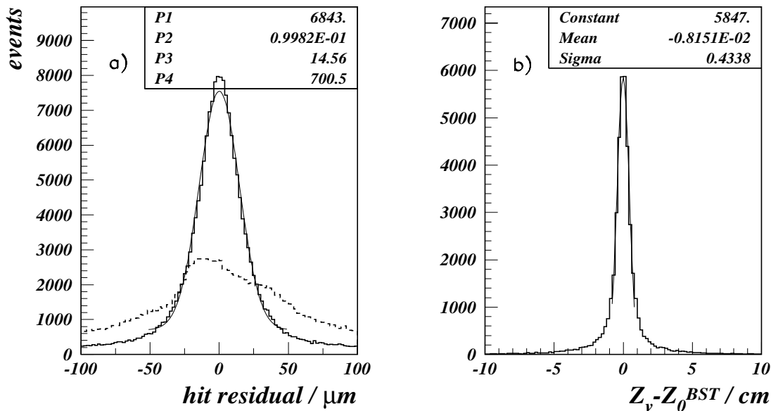
Figure 4.13: Quality of the internal alignment. a) represents the hit residuals for all 64 detectors before (dashed curve) and after (solid histogram) performing the internal alignment. b) shows the difference between the vertex measured with the central tracker detectors requiring its accuracy to be better than 0.3 cm and the one reconstructed with the BST after alignment.
