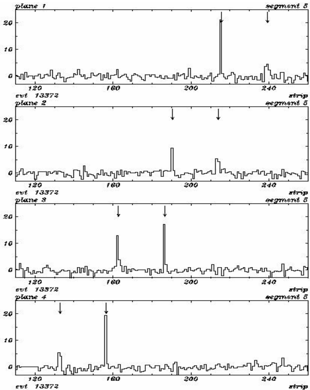
Figure 4.9: An example of an event with the recognized hits induced by two charged particles which crossed the four successive planes of the BST.
