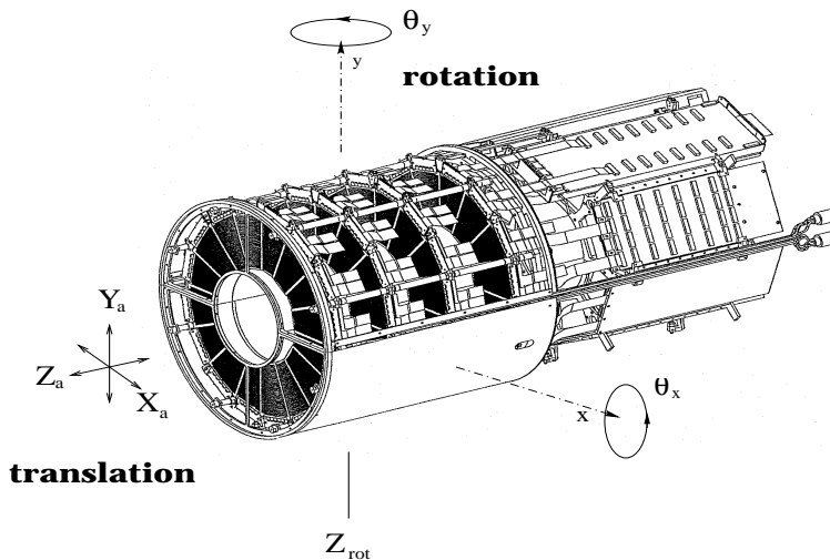
Figure 4.14: Sketch defining the global alignment parameters of the BST. The parameters Y_a , X_a and Z_a stand for translation. A rotation of the BST is parameterized by the two Euler angles \theta_x and \theta_y . The third Euler angle is omitted due to \phi symmetry of the tracker.
