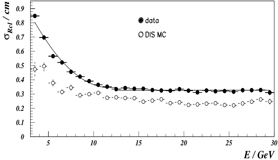
Figure A.2: The SpaCal spatial resolution as a function of electron candidate cluster energy. Closed (open) points represent the spreads of Gaussian fit performed to the distribution of the quantity R_{BDC}^{onSpaCal} - R_{SpaCal} in energy slices for data (DIS Monte Carlo simulation). The larger deterioration in the data may be due to residual \gamma p background in the data sample.
