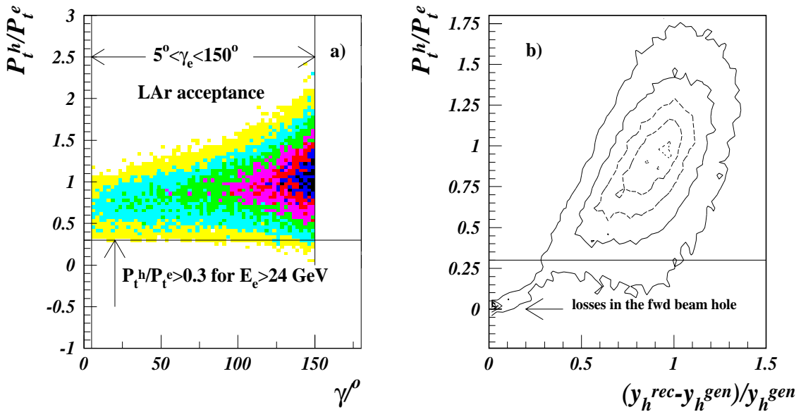
Figure 5.3: a) Some of the cuts imposed to select an event sample with minimized losses or leakage of hadronic energy due to limited acceptance of the LAr calorimeter. Contour lines in figure b) indicate the correlation between the P_t balance ( P_t^h/P_t^e ) and the y_h reconstruction. The solid line represents the P_t balance cut which suppresses the energy losses in the forward beam direction.
