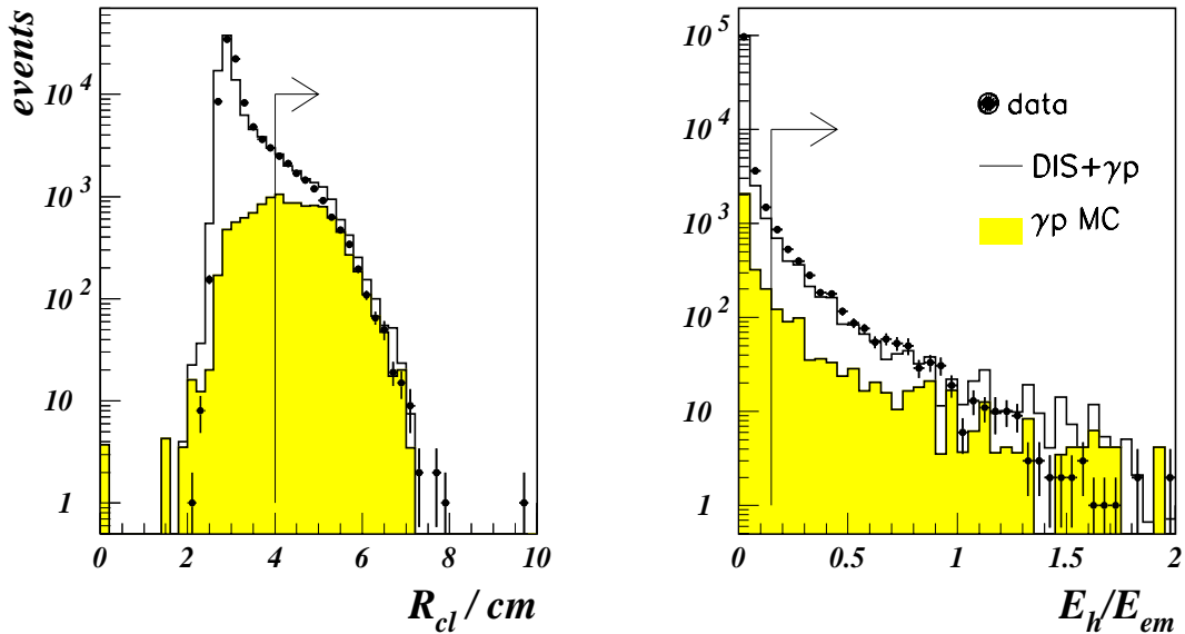
Figure 6.4: Left: cluster radius distribution with logarithmic weighting (see text) presented with energy selection E'_e < 20 GeV. Also shown is the R_{cl} < 4 cm cut. Bulk of the rejected events are clearly related to the \gamma p background. Right: distribution of the E_{had}/E_{em} ratio corresponding to the longitudinal size of the electron candidate cluster. The applied cut on E_{had}/E_{em} < 0.15 is also shown and, as one can see, it rejects mostly hadronic clusters. Closed points correspond to the data, the shaded histograms present the \gamma p background and the open histograms are a sum of a DIS Monte Carlo simulation and the \gamma p background for both pictures.
