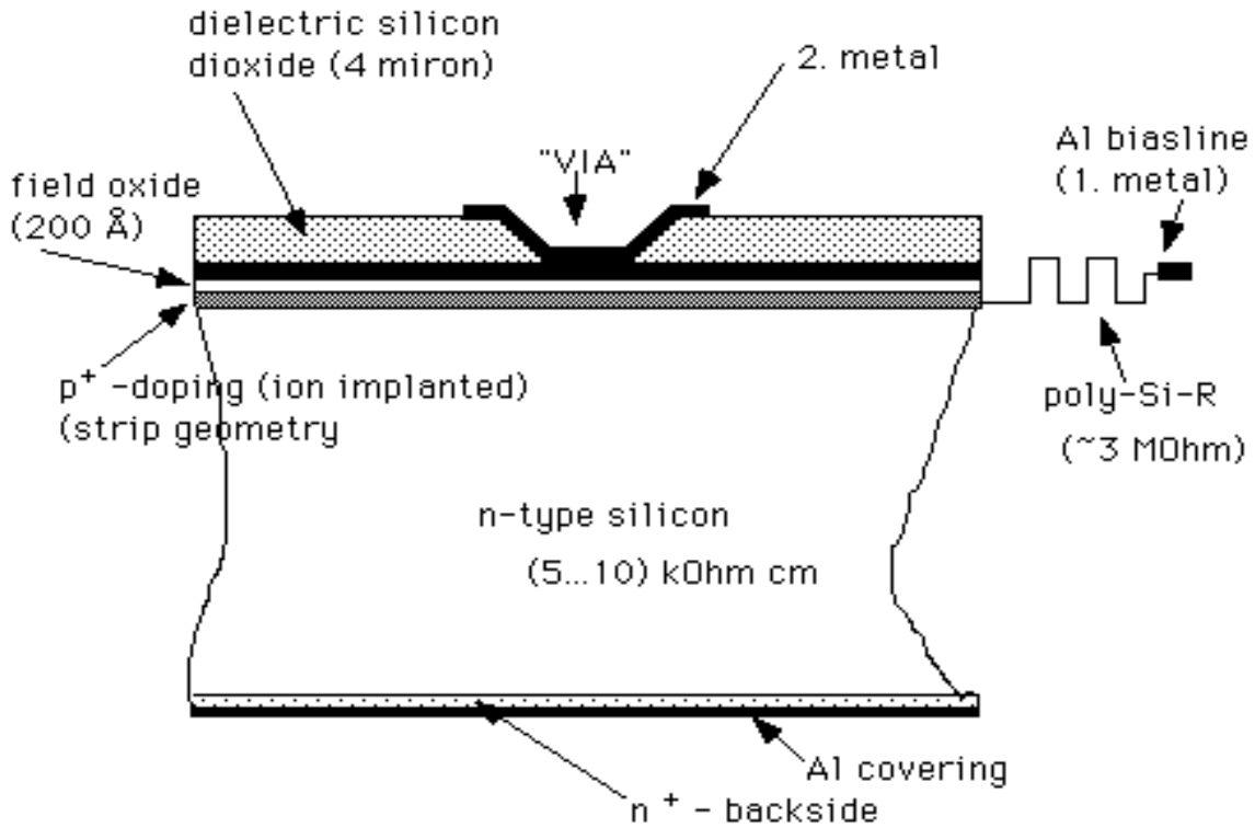
Figure 4.6: Cross section of the single sided, double metal, 300 \mu\text{m} thin silicon p^+ -type strip detector of the BST.
