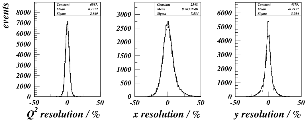
Figure 4.3: The resolution of the kinematic variables in the low Q^2 , high y region with and without using the BST illustrated by the solid and hatched curves, respectively.
