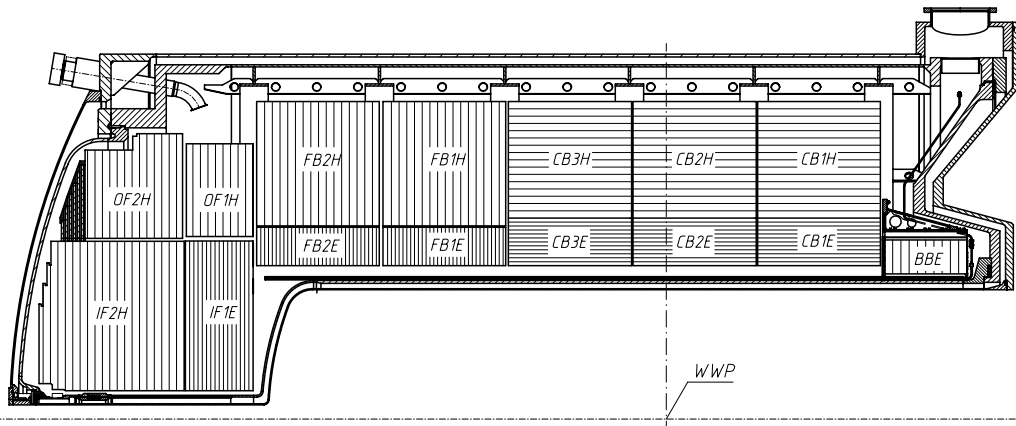
Figure 3.4: Schematic view of the LAr calorimeters.
