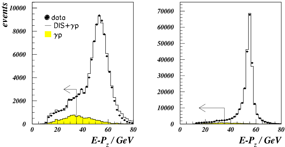
Figure 6.5: Distribution of the quantity E - P_z for energies 5.5 < E'_e < 20 GeV (left picture) and for E'_e > 5.5 GeV (right picture). Closed points present data. The shaded histograms illustrate the simulated \gamma p background. The open histogram is a sum of the DIS Monte Carlo simulation and this background. Both distributions correspond to events with all DIS selection criteria being satisfied, excluding the E - P_z cut itself. The applied cut on E - P_z > 35 GeV is shown on both pictures. The rejected events are well described by the simulation. A drop at E - P_z = 27.6 GeV corresponds to the central vertex requirement for y > 0.5 in order to suppress the QED Compton events (see text).
