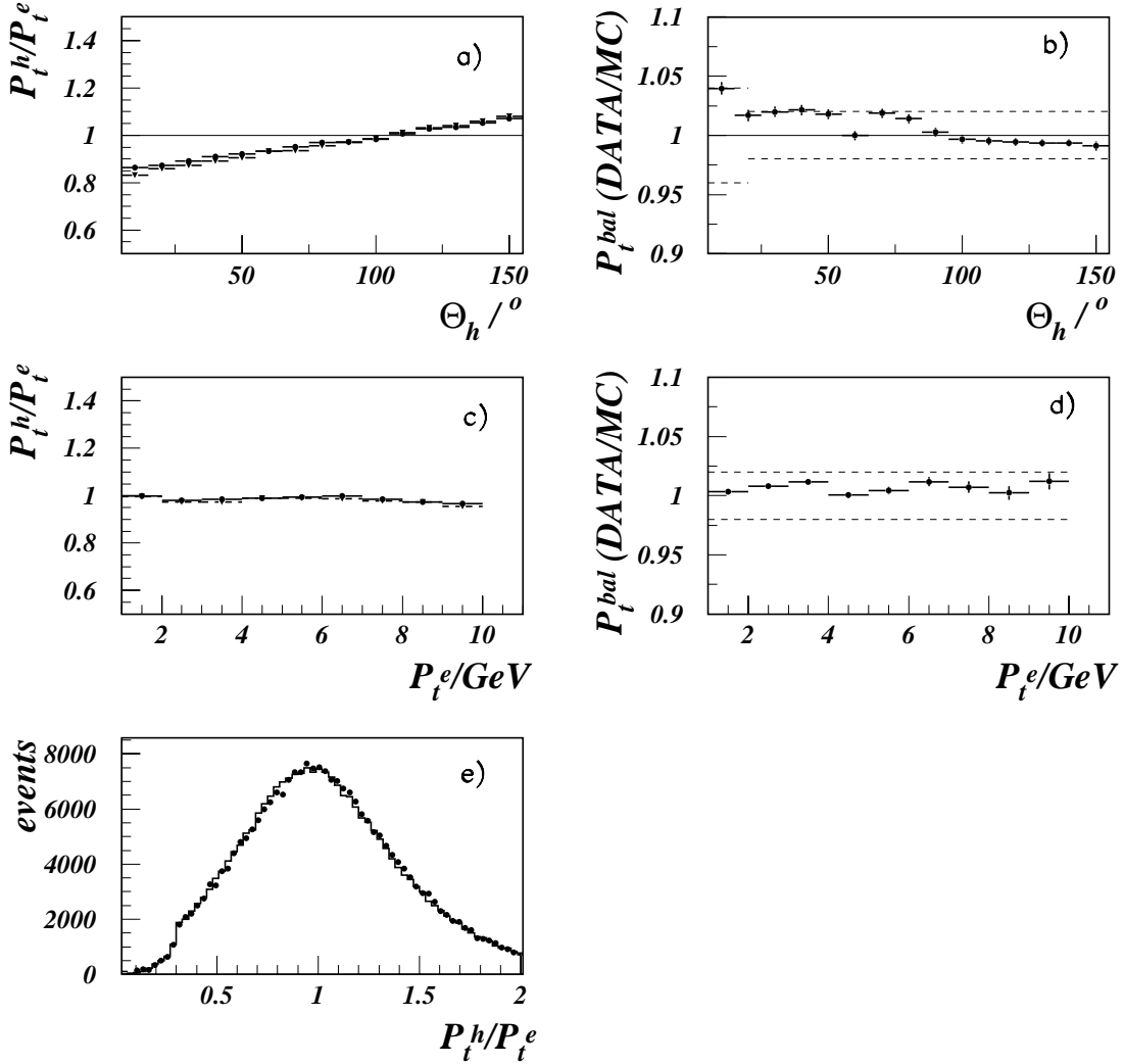
Figure 5.5: Control plots for the LAr calibration with the Lagrangian method. Mean values of the P_t balance as a function of \theta_h (a) and P_t^e (c) for data (closed circles) and Monte Carlo (closed triangles). The corresponding ratios of the mean values between data and Monte Carlo are presented in figures b) and d). Dashed lines in figure b) represent the suggested systematical uncertainty of 2% for backward and central parts of the LAr calorimeter and of 4% for the forward one. The dashed lines in figure d) show that the mean data to Monte Carlo P_t balance ratio is well within 2% variations independently of the transverse momentum of the final state electron. Figure e) represents the shape of the P_t balance which is very well described by Monte Carlo simulation, and both distributions are peaked at unity.
