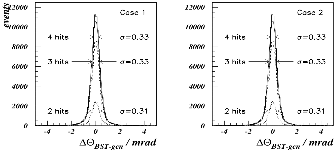
Figure A.5: Comparison of the reconstructed electron polar angle with the generated one performed within the corridor (left figure) and semi-combinatoric (right figure) approach. The comparison is shown for 2, 3 and 4 BST hits defining the electron track.
