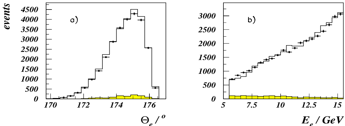
Figure 6.14: Control distributions for the high y kinematical domain ( y > 0.5 ). a) Polar angle and b) energy distributions for the scattered electron measured with the BST and the SpaCal.
