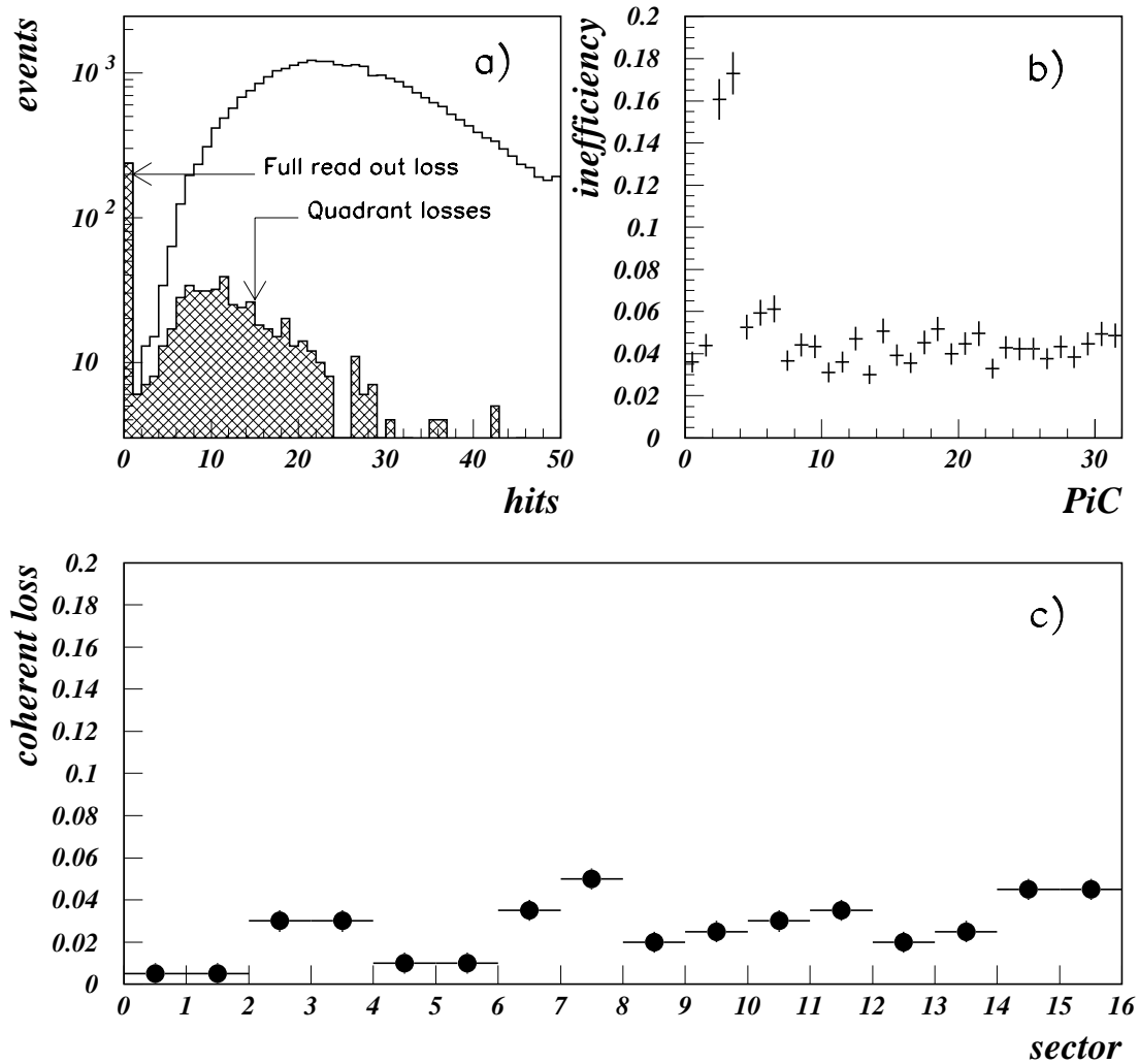
Figure 4.12: a) Distribution of the total number of hits in the BST in case when all four planes are crossed by an electron track (open histogram). The dashed histogram represents the part of events with identified coherent losses either fully or quadrant-wise (see in the text). b) Inefficiency plotted as a function of the number of the storage capacitor in the APC ("pipeline counter PiC"). Two pipeline counters out of thirty two were found to be less efficient resulting in about 0.5% of the coherent losses. The total amount of the coherent losses is presented in plot c) sector-wise.
