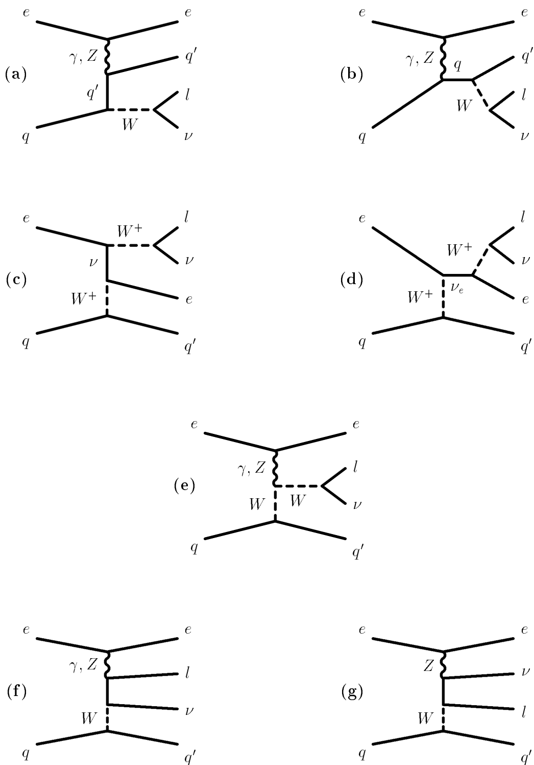
Figure 2.8: Leading order diagrams for W production in the process eq \rightarrow eq'l\nu .
