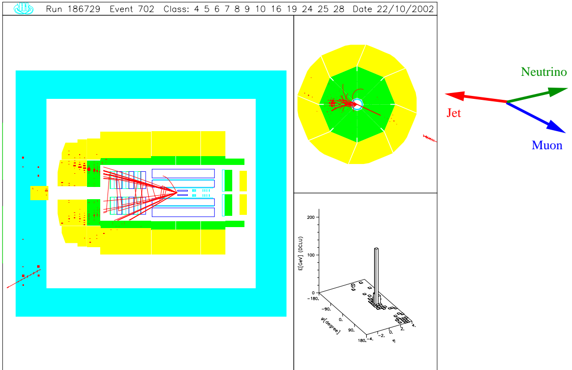
Figure 6.1: Event with a high- P_T muon ( P_T^\mu = 51_{-11}^{+17} GeV), identified by its track in the muon system, and a large missing transverse momentum ( P_T^{\text{miss}} = 28 GeV). The missing transverse momentum becomes obvious as acoplanarity between the muon and the hadronic final state in the transverse plane. This event has a large hadronic transverse momentum of 67 GeV.
