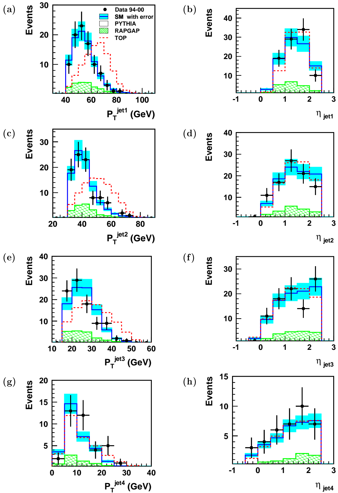
Figure 7.5: Distributions of the jet transverse momenta and pseudorapidities for the selection of multi-jet events with high E_T and a W candidate. The error band corresponds to a 15% uncertainty on the total Standard Model prediction. The top simulation is arbitrarily normalized to the same area as the Standard Model background.
