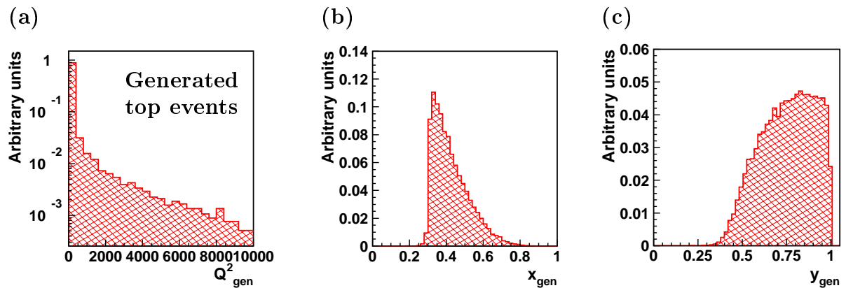
Figure 2.4: Kinematic distributions of generated single top events from FCNC top production at HERA.
