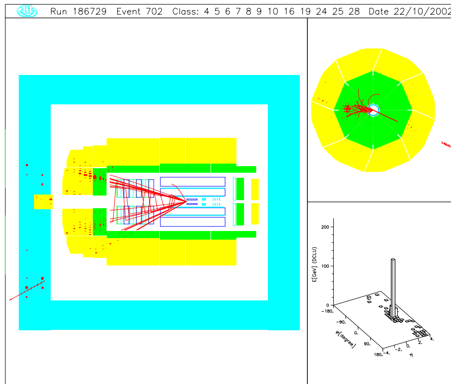
Figure A.10: W \rightarrow \mu^+ \nu candidate. ( top candidate ) P_T^\mu = 51_{-11}^{+17} GeV , P_T^{miss} = 28 GeV , P_T^{jets} = 72 GeV , M_{e-\nu-jets} = 176 GeV.
