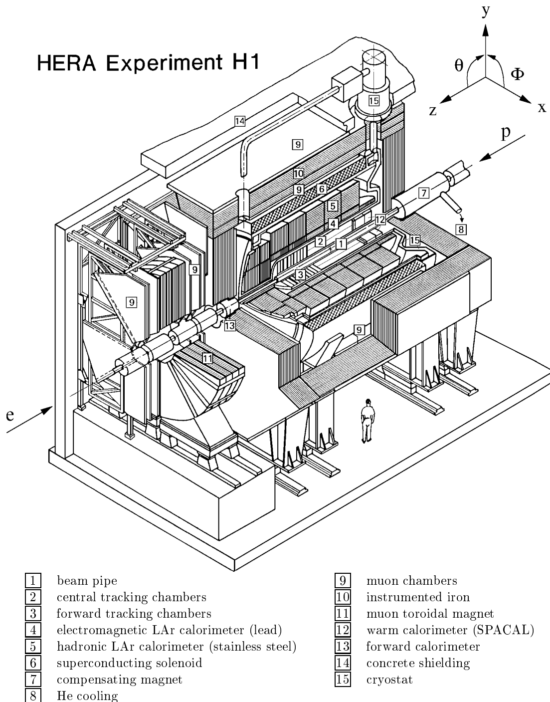
Figure 3.2: The H1-Detector.
