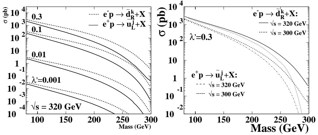
FIGURE 2.14: Cross section for resonant squark production in e^\pm p collisions. Shown are the cross sections as a function of the squark mass for various values of the \mathcal{R}_p coupling \lambda' (left) and for the two centre of mass energies of HERA (right).
