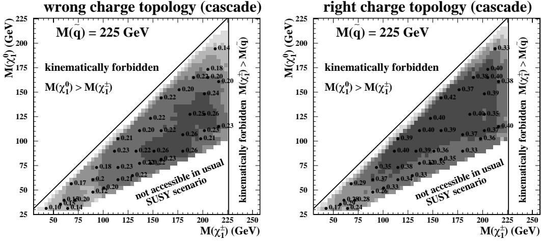
FIGURE 6.11: Selection efficiencies in cascade decays leading to the 'wrong' (left) and 'right' (right) charge topologies ( \tilde{q} \rightarrow q\chi_1^\pm \rightarrow qq\tilde{q}\chi_1^0 \rightarrow qq\tilde{q}e^\pm\tilde{q}q ). Shown are the efficiencies for an example squark mass of 225 GeV.
