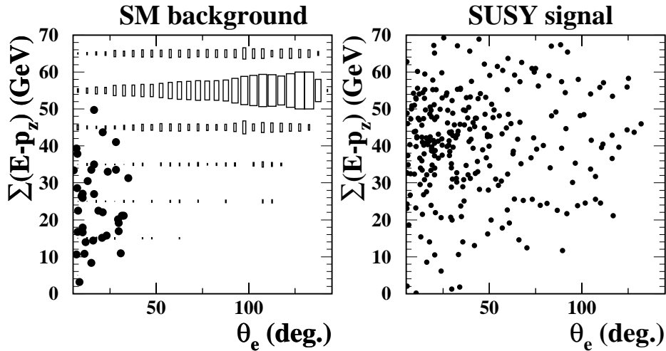
FIGURE 6.2: Distributions of MC events in the (\sum(E-p_z), \theta_e) -plane. In the left panel the SM background is shown: NC DIS (box histogram) and \gamma p (dots, arb. norm.); The right panel illustrates the SUSY signal. Events with low \sum(E-p_z) and electron candidates in the very forward direction are rejected. The SUSY signal is shown for squark decays leading to \nu e M J topologies where the cut should have the biggest effect.
