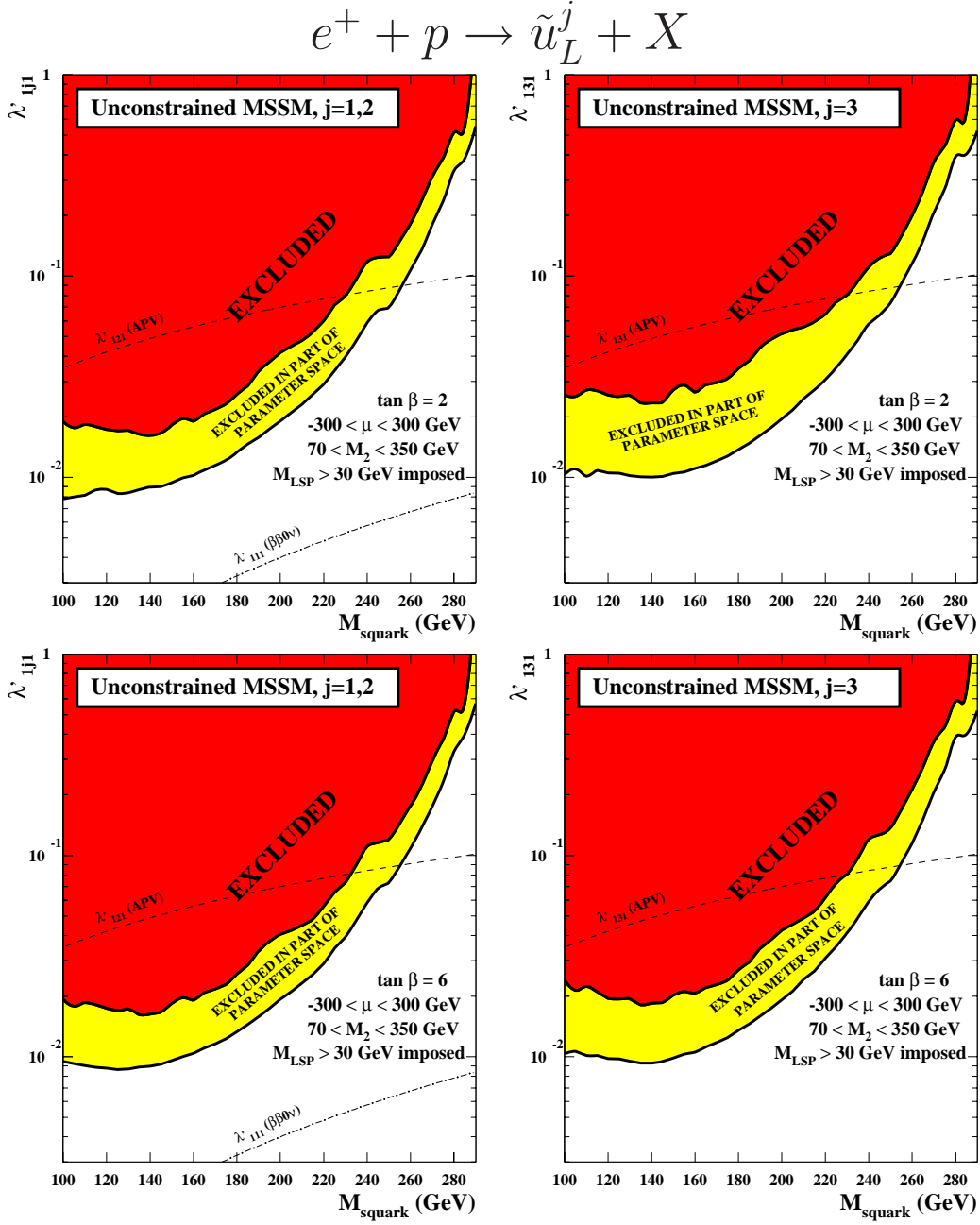
FIGURE 8.6: Exclusion limits (95% CL) on \lambda'_{1j1} for j = 1, 2 (left) and j = 3 (right) as a function of the squark mass for \tan \beta = 2 (top) and for \tan \beta = 6 (bottom) from a scan of the MSSM parameter space as indicated in the figures. The two full curves indicate the strongest and the weakest limits on \lambda' in the parameter space investigated. Indirect limits from neutrinoless double beta decay experiments ( \beta\beta 0\nu ) [12] and atomic parity violation (APV) [13, 14] are also shown.
