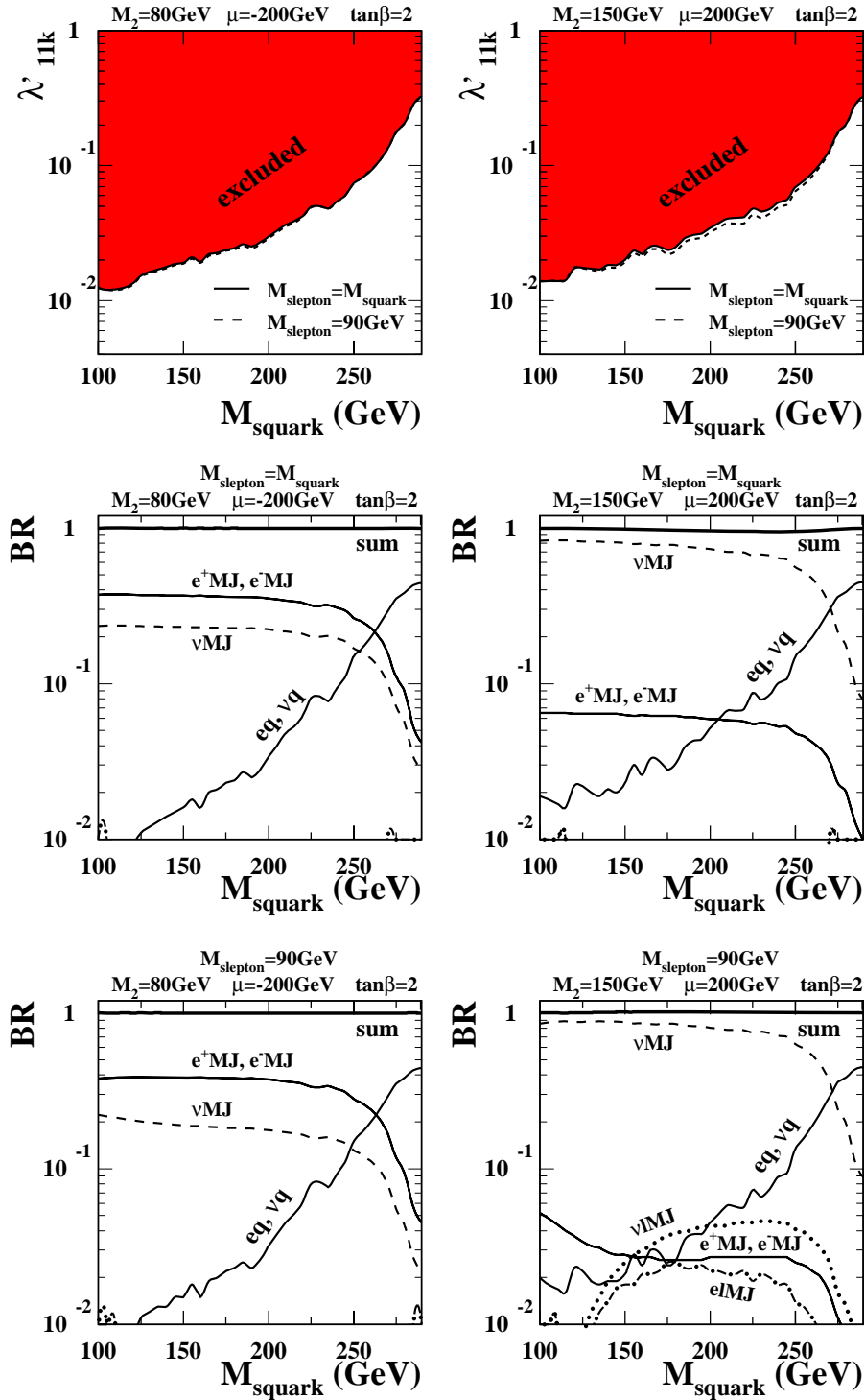
FIGURE 8.4: Exclusion limits (95% CL) on \lambda'_{11k} with k = 1, 2 and the BRs of all channels for \lambda' values just at the shown exclusion limit. Shown are the results for MSSM parameters leading to a \chi_1^0 dominated by its \tilde{\gamma} component ( \mu = -200 \text{ GeV} ) (left) and by its \tilde{Z} component ( \mu = 200 \text{ GeV} ) (right) when sleptons and squarks are assumed to be degenerate and for a slepton mass of 90 GeV.
