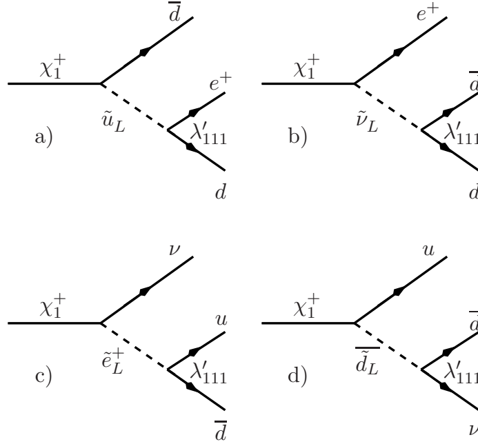
FIGURE 2.17: \tilde{R}_p decay modes of \chi_1^+ for \lambda'_{111} \neq 0 .
