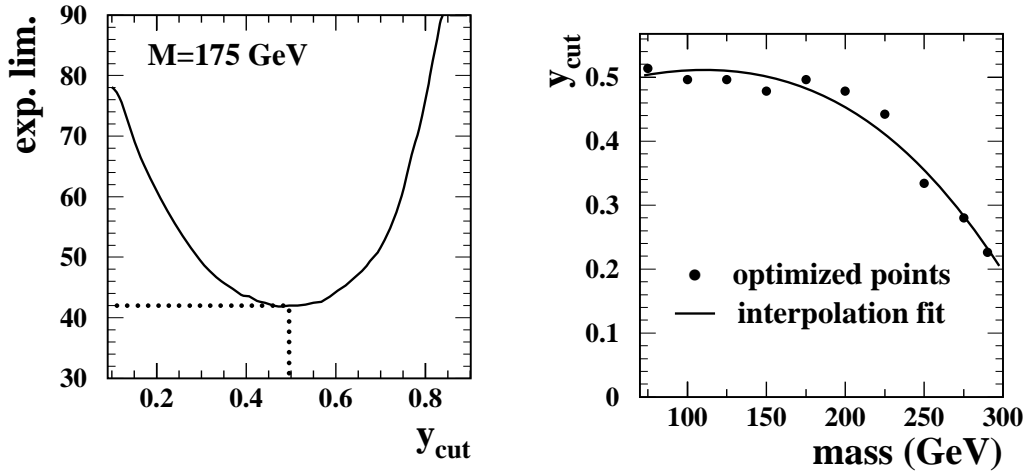
FIGURE 5.4: The expected limit as a function of the lower y_e -cut for a generated squark mass of 175 GeV (left) and the optimized lower y_e -cut for the full mass range (right).
