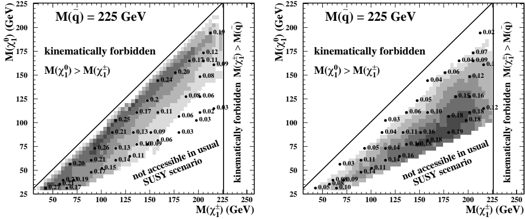
FIGURE 8.1: Cross talk between decay channel and selection channel. Shown are the efficiencies for events from the decay chain \tilde{q} \rightarrow q\chi_{1}^{\pm} \rightarrow q\nu_{\mu}\mu\chi_{1}^{0} \rightarrow q\nu_{\mu}\mu\nu q\bar{q} in the selection channel \nu MJ for an example squark mass of 225 GeV (left). The right panel illustrates the efficiency for \tilde{q} \rightarrow q\chi_{1}^{\pm} \rightarrow q\nu_{e}\chi_{1}^{0} \rightarrow q\nu_{e}e q\bar{q} in the \nu_e MJ selection.
