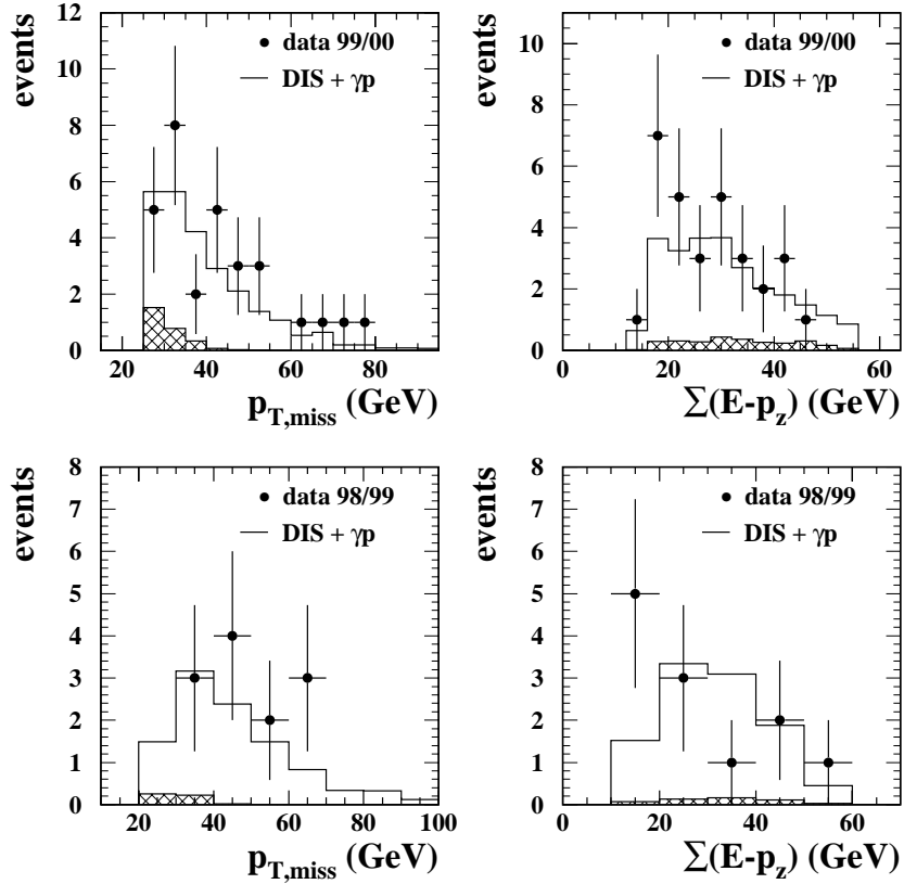
FIGURE 7.1: Control distributions after the \nu MJ preselection in 1999/2000 (top) and 1998/1999 (bottom). Shown are the missing transverse momentum p_{T,\text{miss}} (left) and the momentum balance with respect to the direction of the incident electron \sum(E - p_z) (right). The SM background includes NC DIS, CC DIS and photoproduction (hatched histograms).
