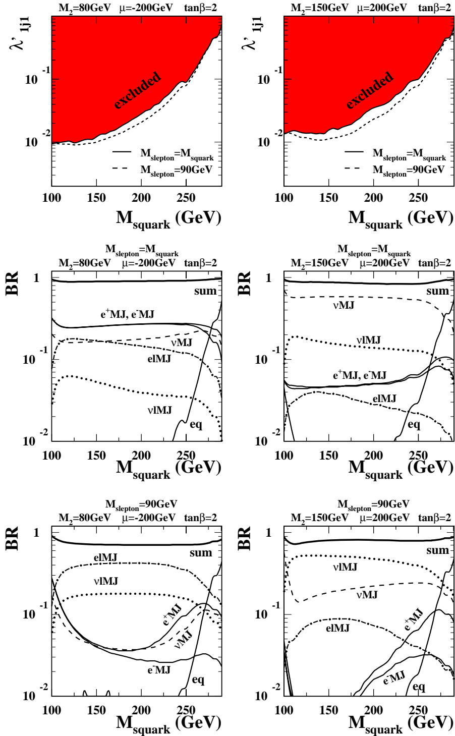
FIGURE 8.3: Exclusion limits (95% CL) on \lambda'_{1j1} with j = 1, 2 and the BRs of all channels for \lambda' values just at the shown exclusion limit. Shown are the results for MSSM parameters leading to a \chi_1^0 dominated by its \tilde{\gamma} component ( \mu = -200\text{GeV} ) (left) and by its \tilde{Z} component ( \mu = 200\text{GeV} ) (right) when sleptons and squarks are assumed to be degenerate and for a slepton mass of 90 GeV.
