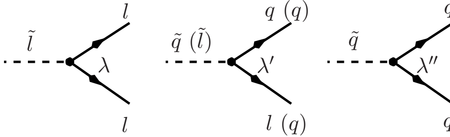
FIGURE 2.8: Diagrams corresponding to R_p violating terms described by Eq. 2.33. \lambda_{ijk}L_iL_j\bar{E}_k (left); \lambda'_{ijk}L_iQ_j\bar{D}_k (middle); \lambda''_{ijk}\bar{U}_i\bar{D}_j\bar{D}_k (right). The process in the middle is of particular interest in ep collisions.
