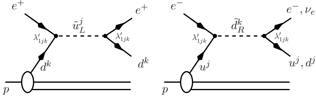
FIGURE 2.15: Feynman diagrams for R_p squark production at HERA followed by R_p squark decays for \lambda'_{1jk} \neq 0 .
