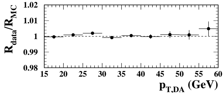
FIGURE 4.6: Dependence of the electron calibration on the transverse momentum. Shown is the ratio R_{\text{data}}/R_{\text{MC}} with R_{\text{data}} and R_{\text{MC}} being the fitted mean of the (p_{T,e}/p_{T,DA}) distribution in the corresponding p_{T,DA} range for data and MC respectively.
