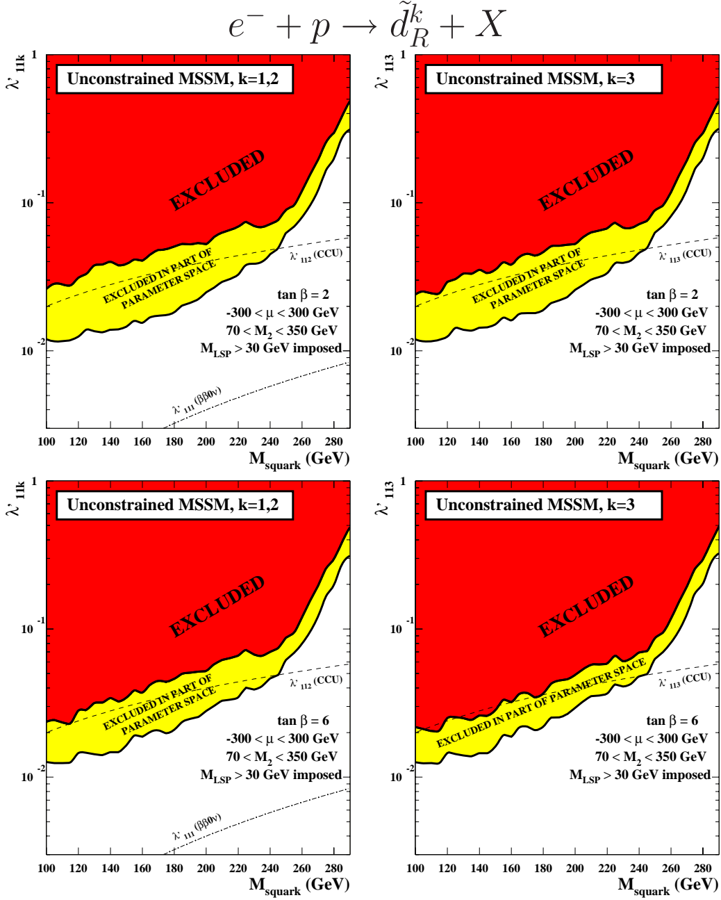
FIGURE 8.7: Exclusion limits (95% CL) on \lambda'_{11k} for k = 1, 2 (left) and k = 3 (right) as a function of the squark mass for \tan \beta = 2 (top) and for \tan \beta = 6 (bottom) from a scan of the MSSM parameter space as indicated in the figures. The two full curves indicate the strongest and the weakest limits on \lambda' in the parameter space investigated. Indirect limits from neutrinoless double beta decay experiments ( \beta\beta 0\nu ) [12] and charged current universality (CCU) [14] are also shown.
