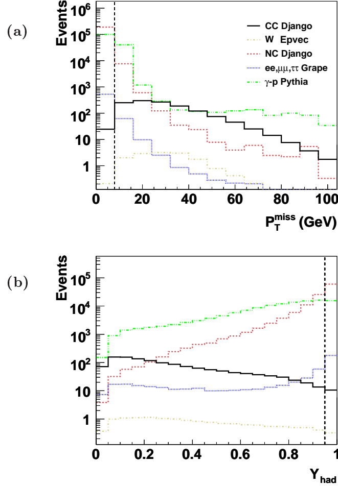
Figure 5.2: The p_{T,miss} (a) and y_h (b) distributions for the simulated charged current events and simulated background processes (see section 1.4) for Q_h > 100 \text{ GeV}^2 . The preselection cuts ( p_{T,miss} > 8 \text{ GeV} and y_h < 0.95 ) are indicated in the plots.
