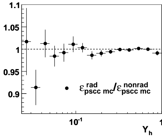
Figure 5.18: Ratio of the vertex requirement efficiencies determined from PSCC MC generated ignoring photon radiation off the lepton line and the usual radiative PSCC (i.e. NC) simulated events.
