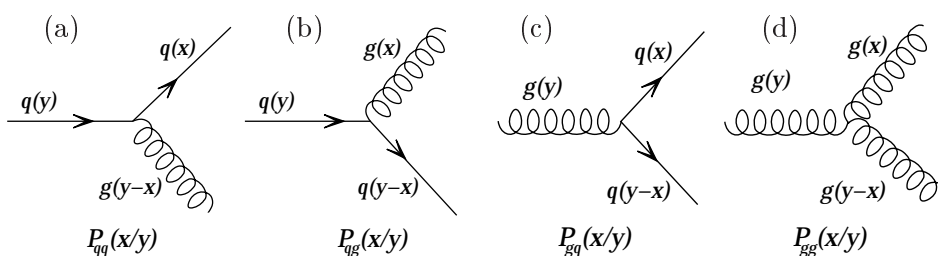
Figure 1.4: Feynman diagrams for each of the four splitting functions P_{ij} and the corresponding elementary processes: (a)-(b) gluon emission by a quark, (c) quark-antiquark creation, (d) gluon emission by a gluon.
