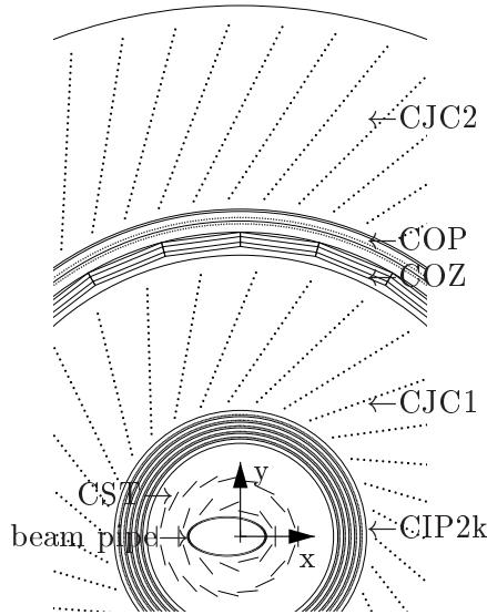
Figure 2.11: The radial view of the Central Track Detector.
