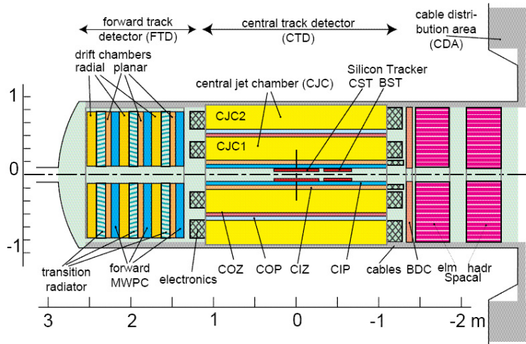
Figure 2.10: The side view of the H1 tracking system. For HERA II, CIZ and part of the CIP chamber are replaced by CIP2k.
