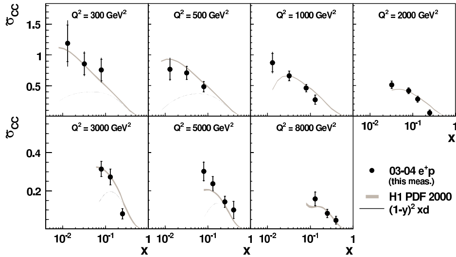
Figure 7.11: Unpolarised e^+p reduced charged current cross sections as function of x for various values of Q^2 (same this analysis data as in Figure 7.9). Also shown are the expected contribution of the valence quark ( xd ) indicated as a dark line. The model uncertainty (H1 PDF 2000) is shown as a shaded band.
