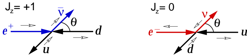
Figure 1.7: Illustration of the angular dependence in charged current reactions (in the CM frame, assuming the z direction along the e^\pm motion and \theta being the scattering angle of the \nu ): (left) the angular momentum component J_z is not conserved if the \bar{\nu} is scattered backwards, i.e. the interaction amplitude is proportional to (1 - \cos \theta) ; (right) the interaction amplitude does not depend on \theta because J_z = 0 .
