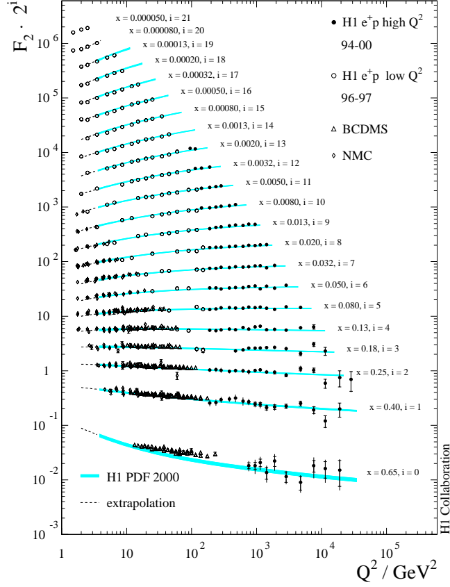
Figure 1.2: Structure function F_2 as function of Q^2 for different x regions. The points represent H1 measurements which are compared with the H1 fit for the proton density functions [18] (band). The measurements of two fixed target experiments (BCDMC [19] and NMC [20]) are also included in the graph.
