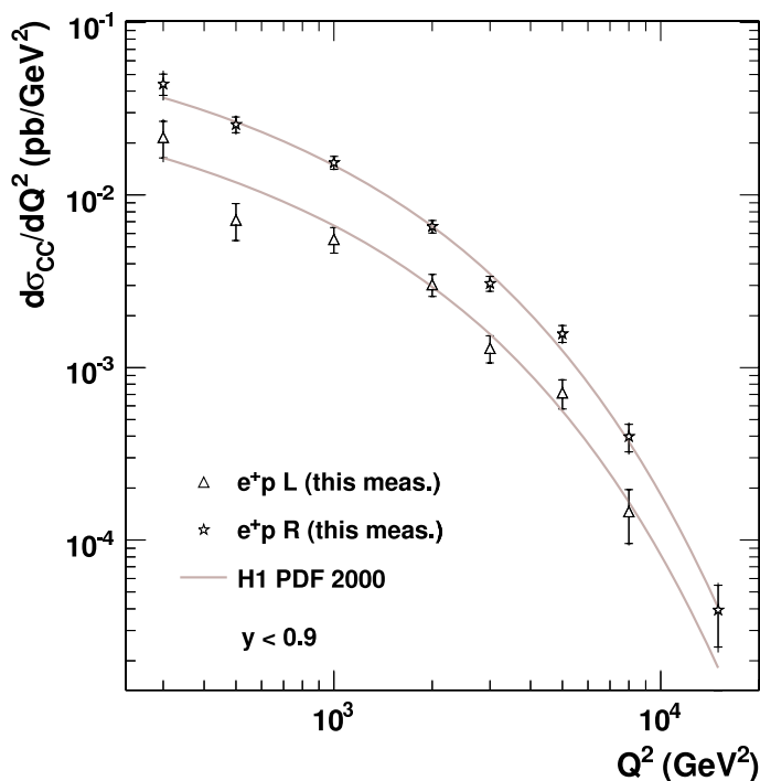
Figure 7.3: e^+p CC cross sections of two polarised ( L and R ) measurements as function of Q^2 for y < 0.9 . For comparison, the SM predictions based on the H1 PDF 2000 parton distribution functions are shown.
