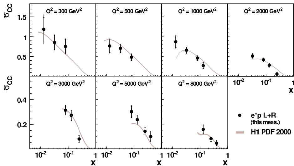
Figure 7.9: Unpolarised e^+p reduced charged current cross section as function of x for different values of Q^2 . The model uncertainty based on the H1 PDF 2000 parton density functions is shown as the shaded band (determined as explained in Figure 7.6).
