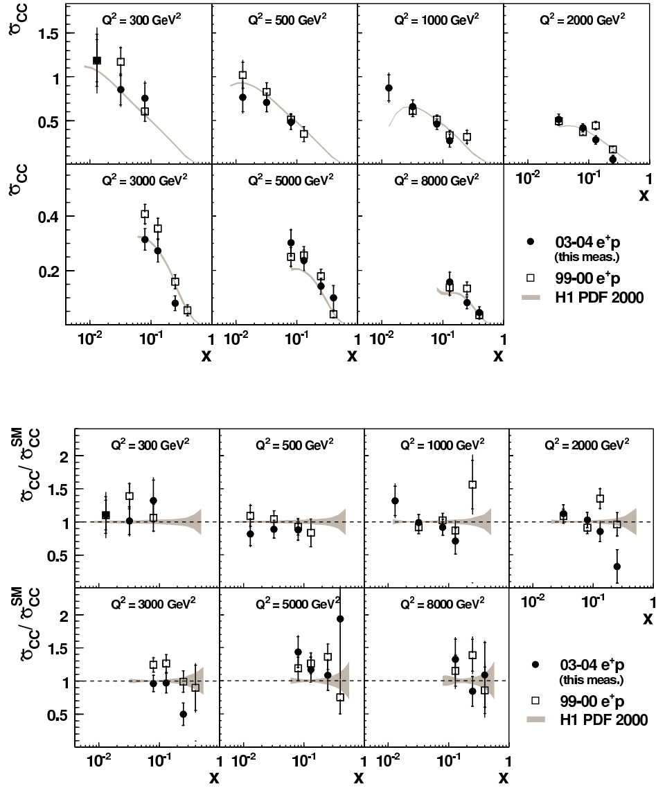
Figure 7.10: Reduced unpolarised e^+p charged current cross section \tilde{\sigma}_{CC} of the present measurement (solid symbols) and previous H1 measurement published in [18] (open symbols) as function of x at different values of Q^2 . The theory expectations based on the H1 PDF 2000 parton distribution functions are shown as bands (determined as explained in Figure 7.6).
