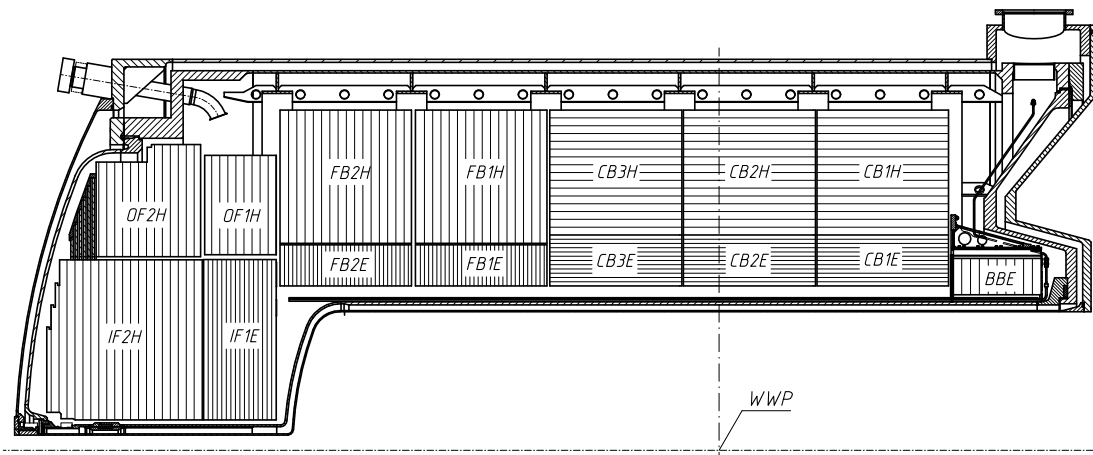
Figure 3.4: Side view of the liquid argon calorimeter. Visible are the eight electromagnetic and the hadronic modules. The modules which are labeled with 'E' correspond to the electromagnetic section and the parts labeled with 'H' to the hadronic section.
