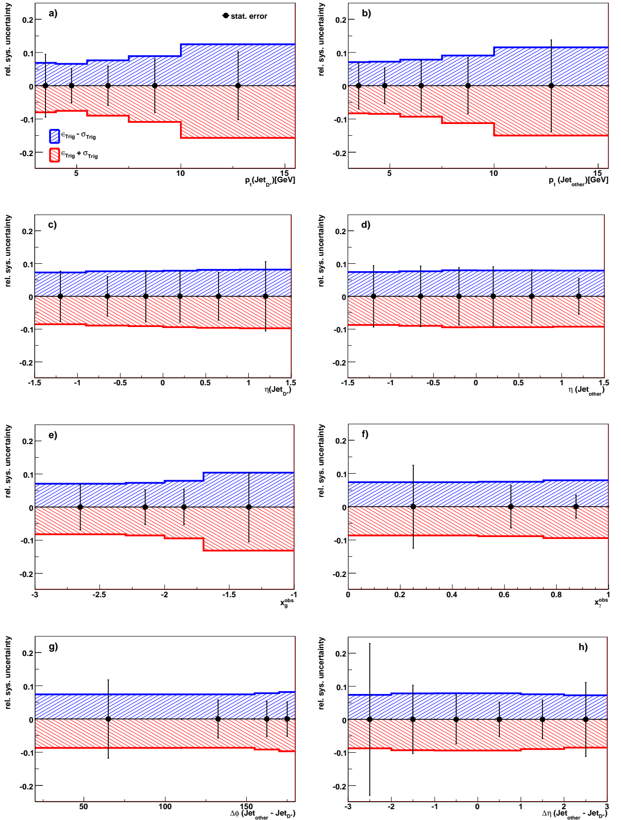
Figure 9.10: Bin by bin uncertainties due to trigger efficiency as a function of the quantities measured in the DiJet sample. The uncertainties have been estimated on the basis of the Pythia (massless) simulation. For details see section 7.
