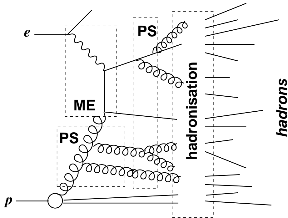
Figure 2.7: Schematic overview of an event generator. Depicted is the hard matrix element ( ME ), initial and final state radiation are incorporated by parton showers ( PS ). The last step is the hadronisation.
